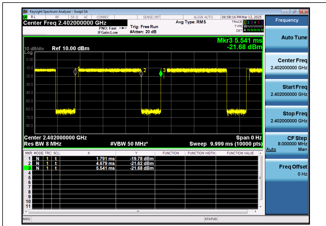
EDR--8DPSK-ANT1-2402
