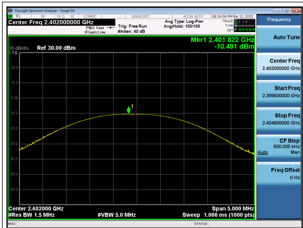
Test_Graph_BR_ANT1_2402_1Mbps_Peak Power
