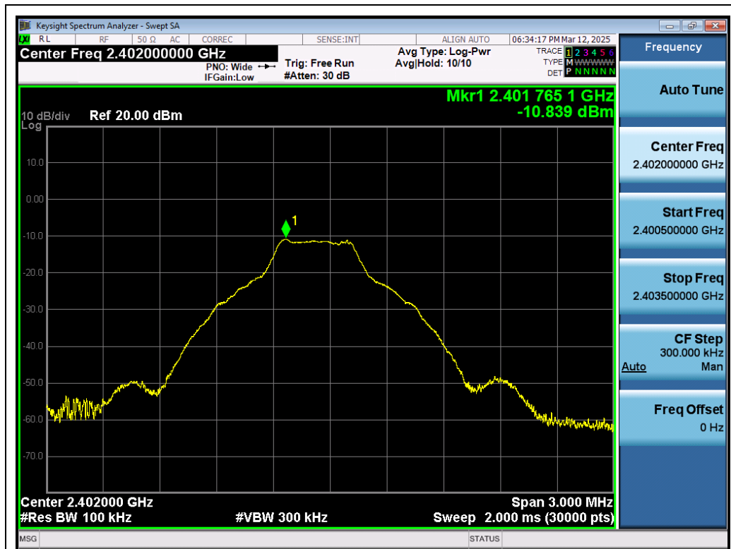
Test_Graph_BR_ANT1_2402_1Mbps_Reference Level
