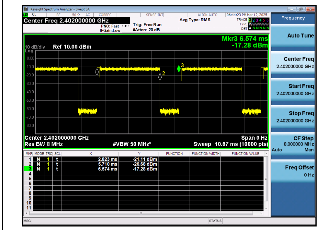
EDR-π /4-DQPSK-ANT1-2402
