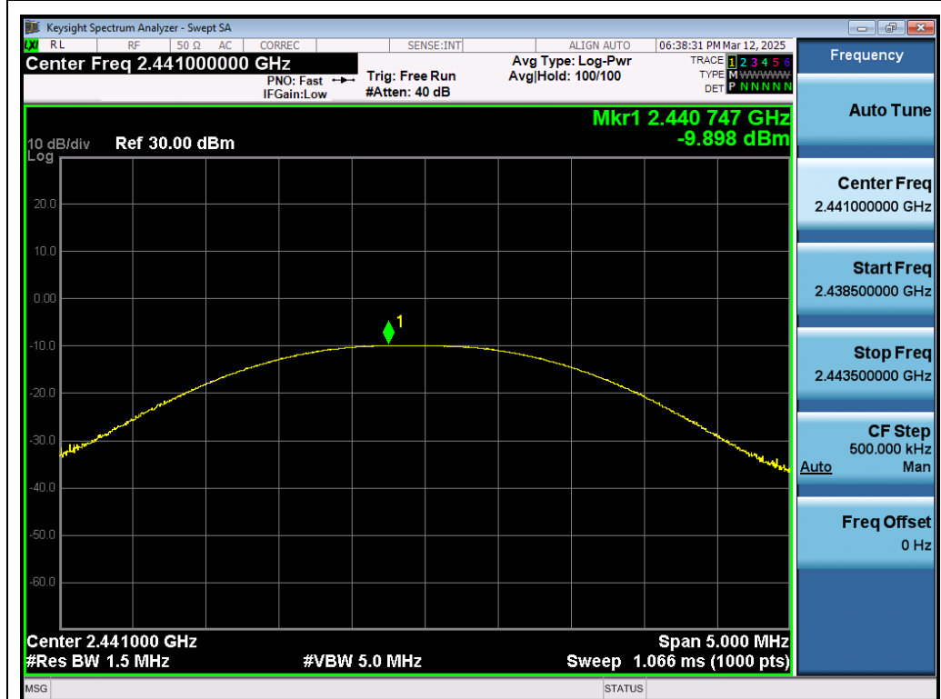
Test_Graph_BR_ANT1_2441_1Mbps_Peak Power
