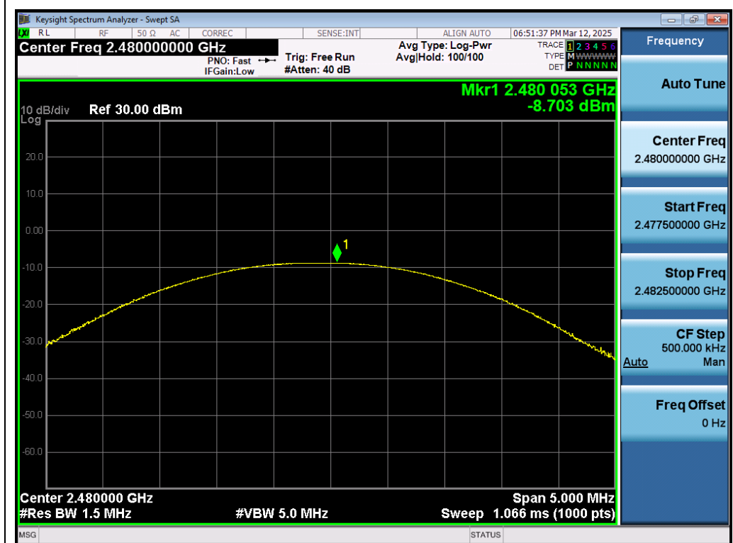
Test_Graph_EDR_ANT1_2480_2Mbps_Peak Power
