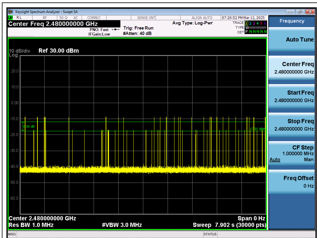
Test_Graph_EDR_HOP_ANT1_NA_3Mbps_2480_Number of Busrt
