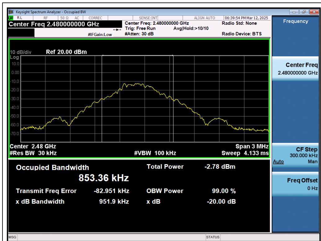
Test_Graph_BR_ANT1_2480_1Mbps_OBW
