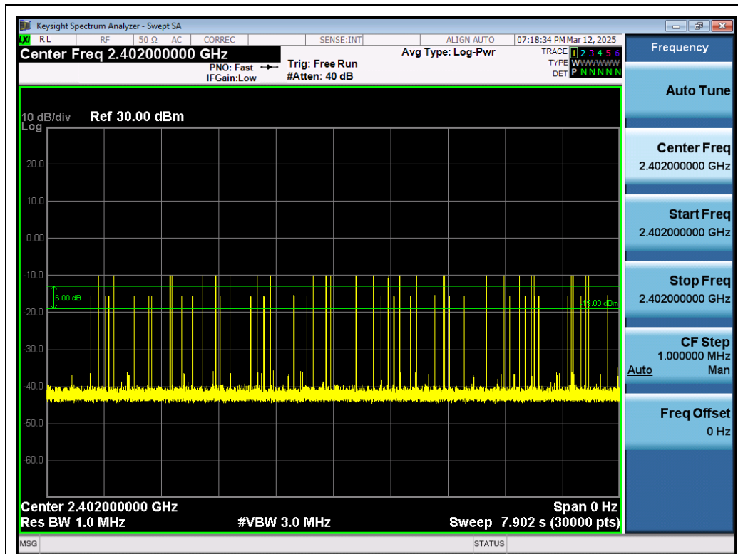
Test_Graph_EDR_HOP_ANT1_NA_3Mbps_2402_Number of Busrt
