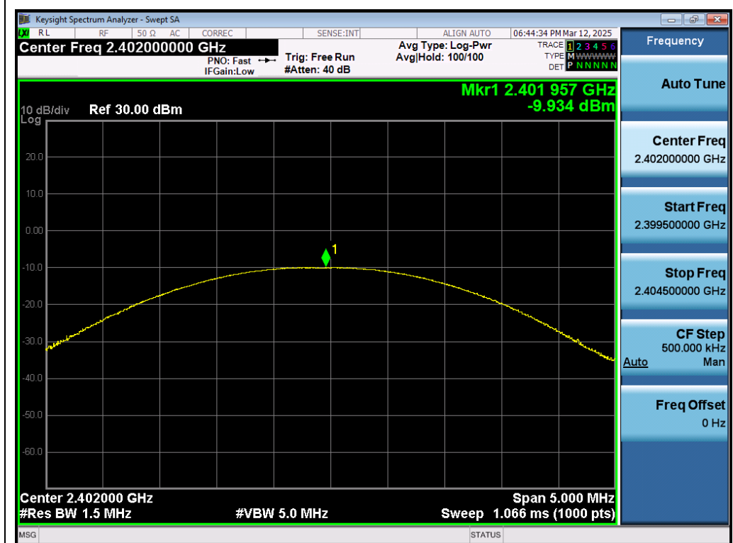
Test_Graph_EDR_ANT1_2402_2Mbps_Peak Power
