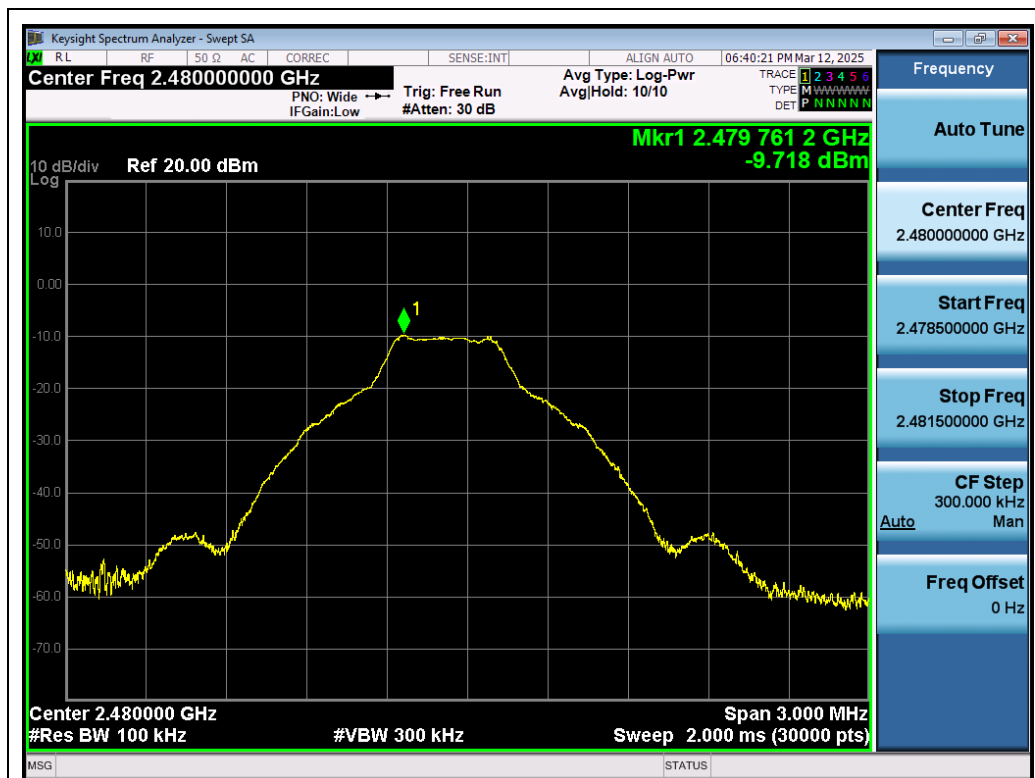
Test_Graph_BR_ANT1_2480_1Mbps_Reference Level
