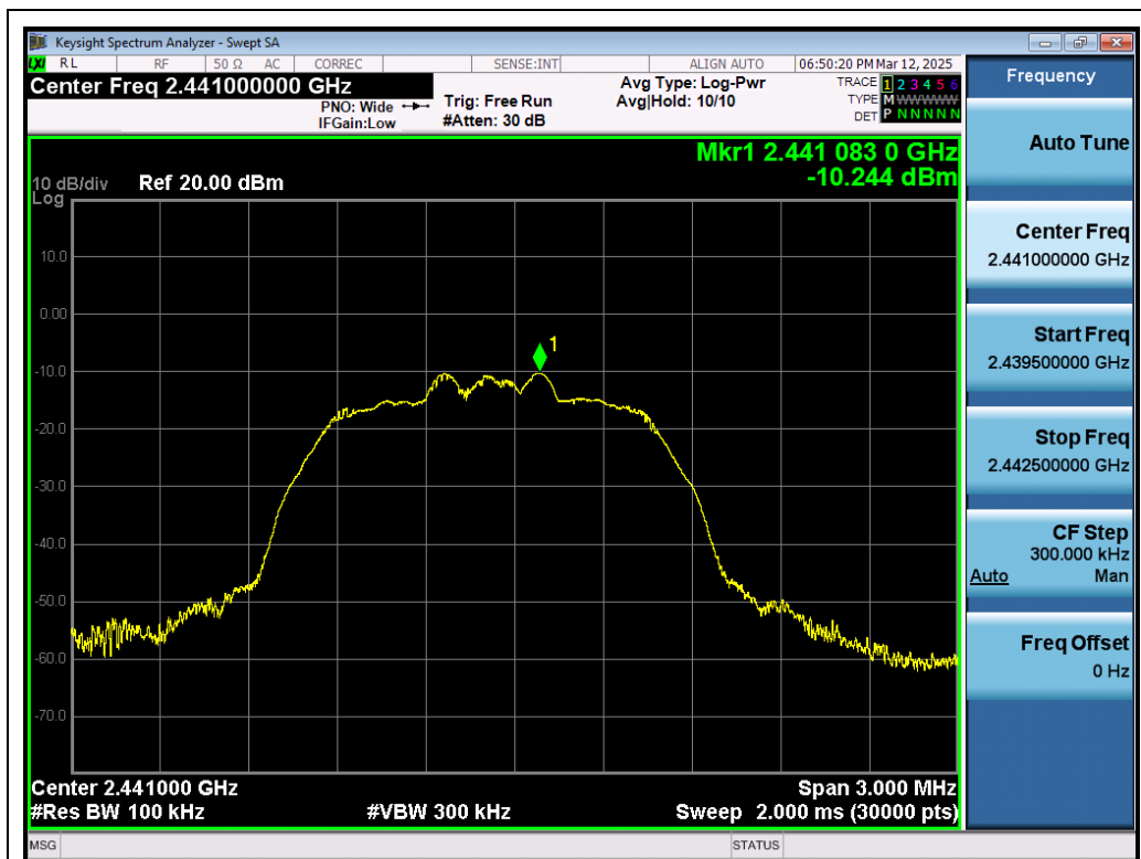
Test_Graph_EDR_ANT1_2441_2Mbps_Reference Level
