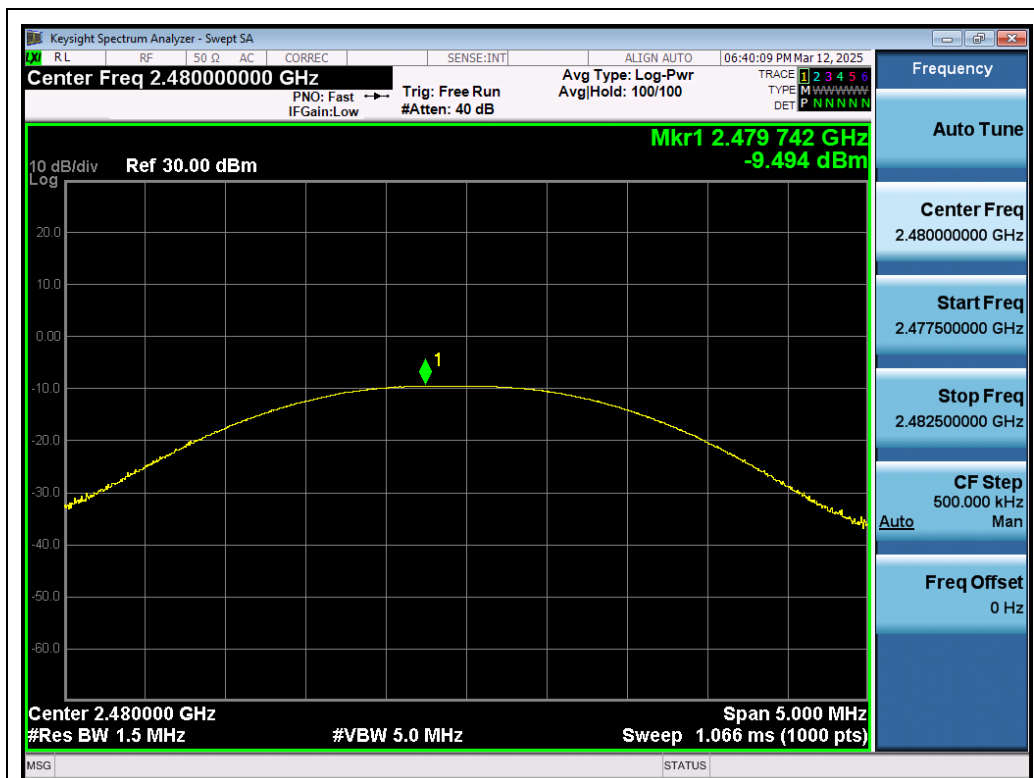
Test_Graph_BR_ANT1_2480_1Mbps_Peak Power
