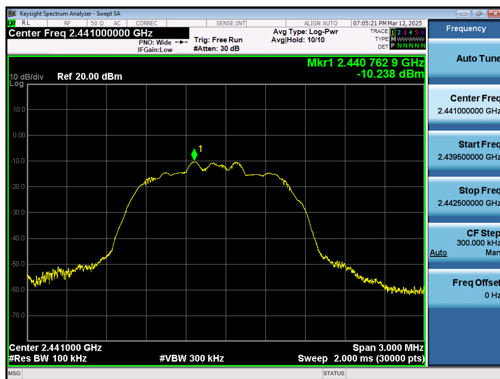
Test_Graph_EDR_ANT1_2441_3Mbps_Reference Level
