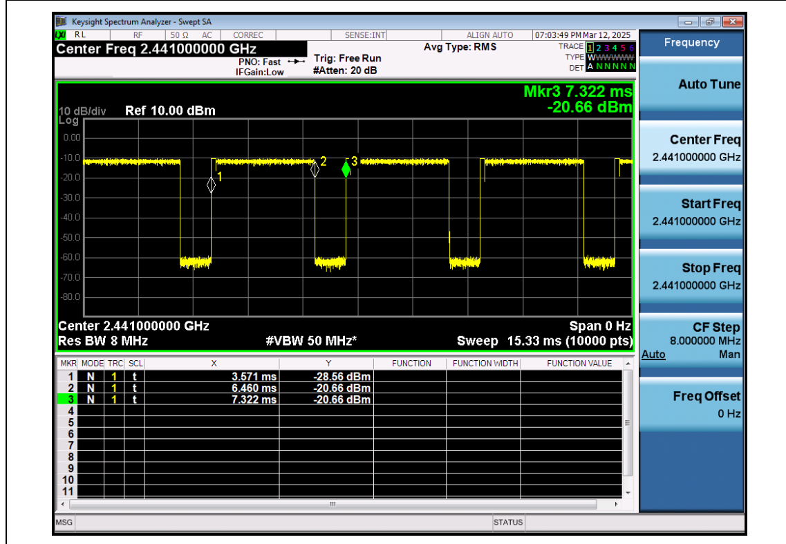
EDR-8DPSK-ANT1-2441
