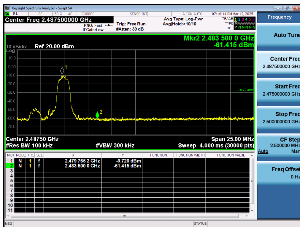
Test_Graph_EDR_ANT1_2480_3Mbps_Higher Band Edge Emissions
