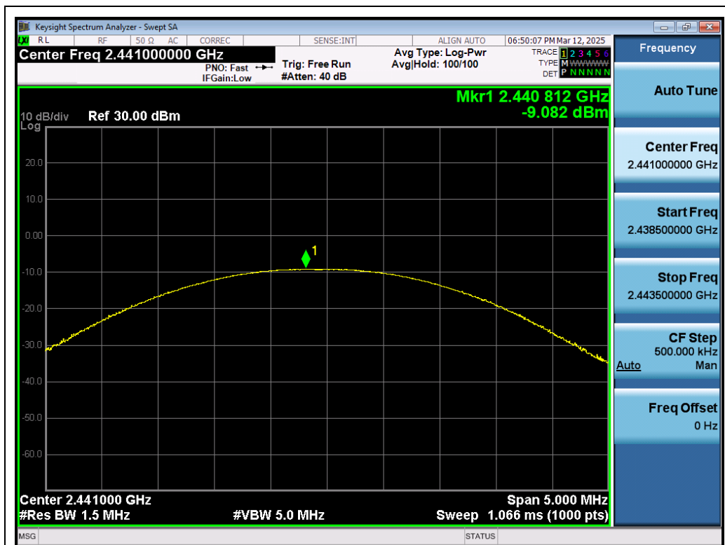
Test_Graph_EDR_ANT1_2441_2Mbps_Peak Power
