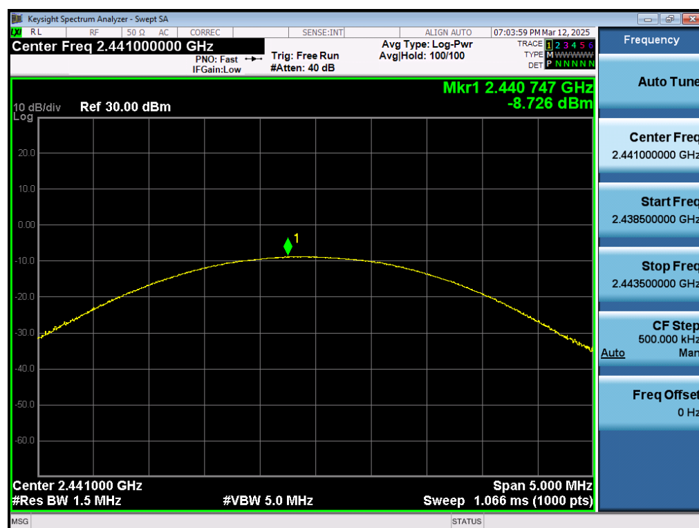
Test_Graph_EDR_ANT1_2441_3Mbps_Peak Power
