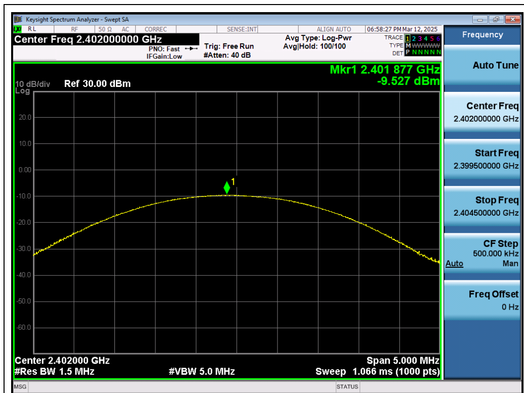
Test_Graph_EDR_ANT1_2402_3Mbps_Peak Power
