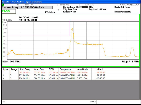
Band 17 5MHz/706.5/Low 16QAM 1@0
