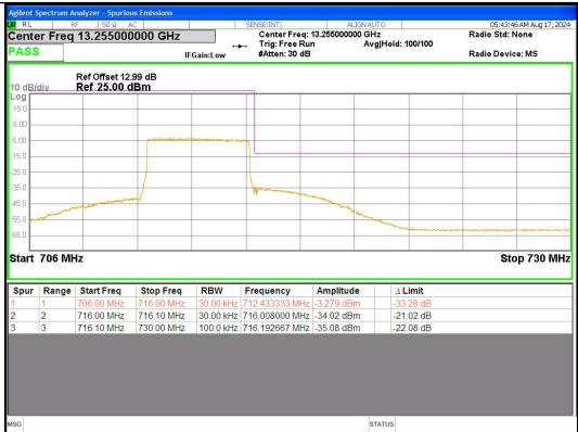
Band 17 5MHz/713.5/High 16QAM 25@0
