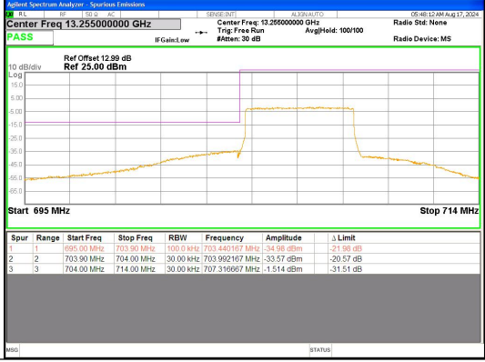
Band 17 5MHz/706.5/Low 16QAM 25@0
