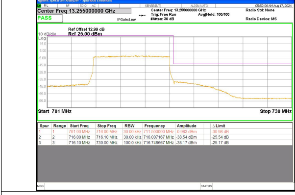
Band 17 10MHz/711.0/High QPSK 50@0
