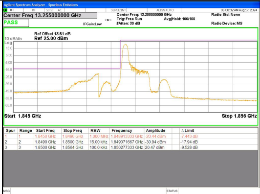
Band 25 1.4MHz/1850.7/Low QPSK 1@0
