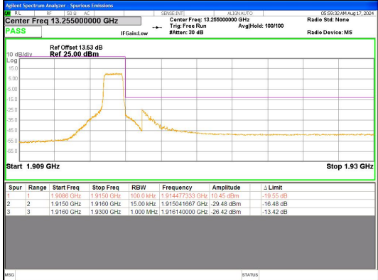
Band 25 1.4MHz/1914.3/High 16QAM 6@0
