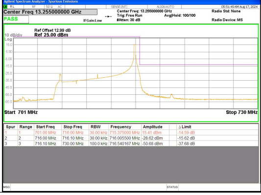
Band 17 10MHz/711.0/High QPSK 1@49
