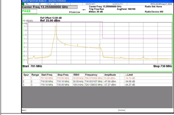
Band 17 10MHz/711.0/High QPSK 1@0
