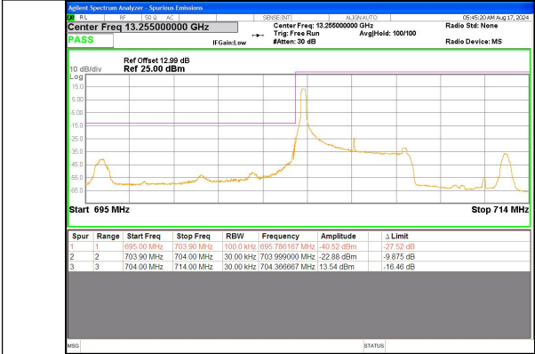
Band 17 5MHz/706.5/Low QPSK 1@0
