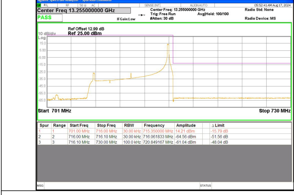
Band 17 10MHz/711.0/High 16QAM 1@49
