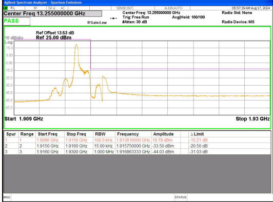
Band 25 1.4MHz/1914.3/High QPSK 1@0
