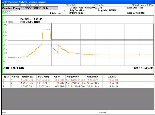
Band 25 1.4MHz/1914.3/High QPSK 6@0
