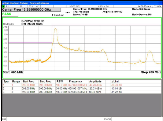
Band 12 5MHz/701.5/Low 16QAM 1@0
