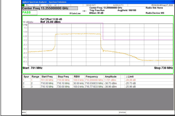
Band 12 10MHz/711.0/High QPSK 50@0
