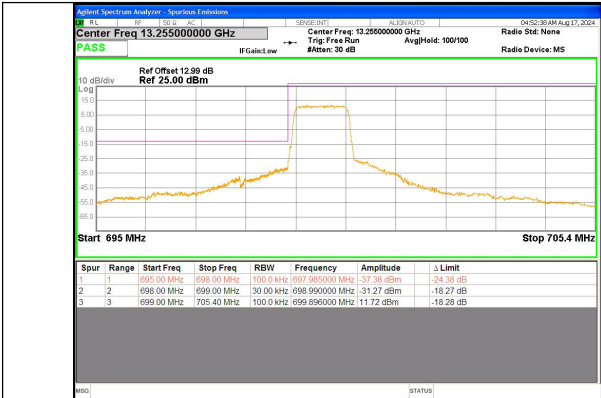
Band 12 1.4MHz/699.7/Low QPSK 6@0
