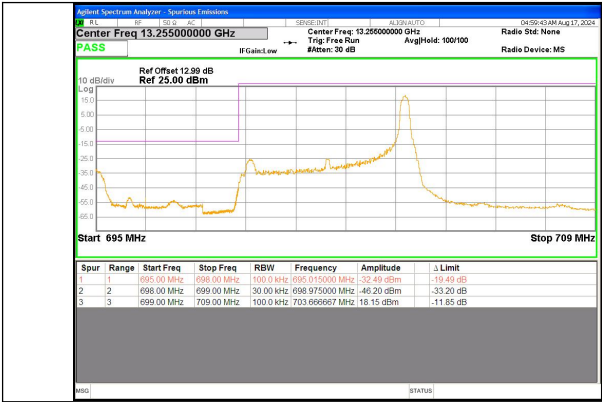
Band 12 5MHz/701.5/Low 16QAM 1@24
