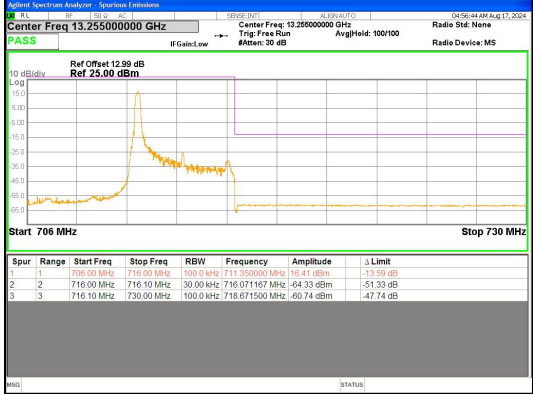
Band 12 5MHz/713.5/High 16QAM 1@0
