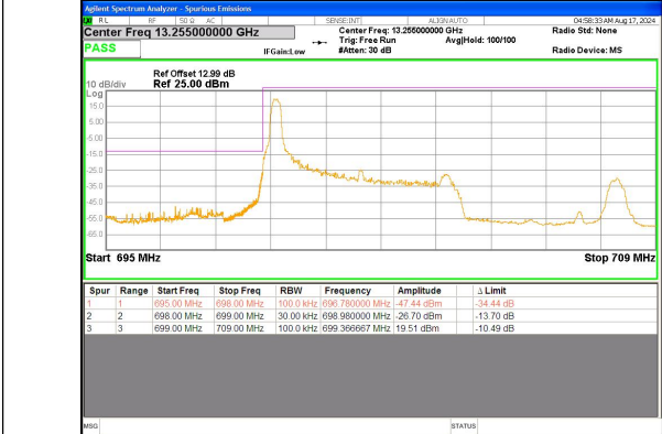
Band 12 5MHz/701.5/Low QPSK 1@0
