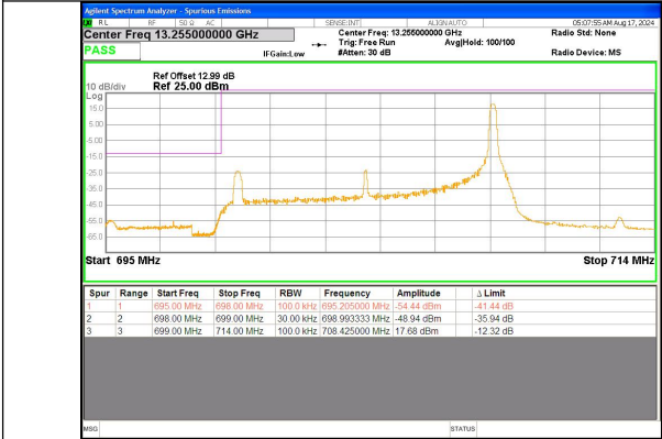
Band 12 10MHz/704.0/Low 16QAM 1@49
