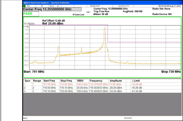
Band 12 10MHz/711.0/High 16QAM 1@49
