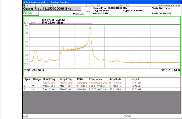
Band 12 5MHz/713.5/High 16QAM 1@24
