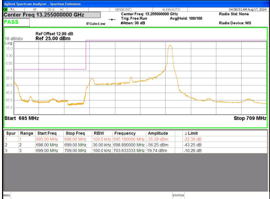
Band 12 5MHz/701.5/Low QPSK 1@24
