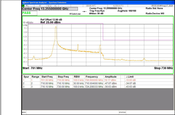
Band 12 10MHz/711.0/High QPSK 1@0
