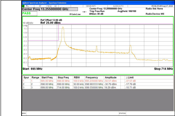
Band 12 10MHz/704.0/Low QPSK 1@0
