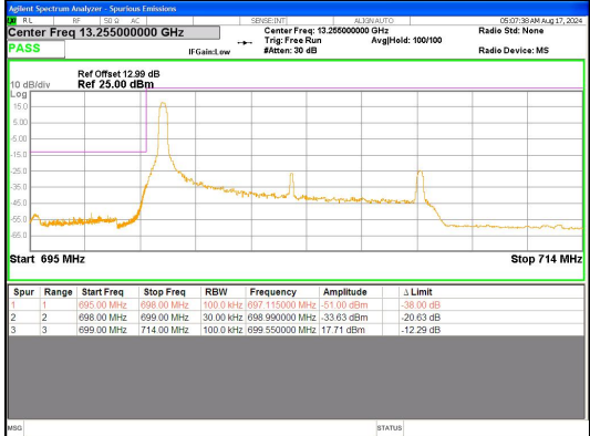
Band 12 10MHz/704.0/Low 16QAM 1@0
