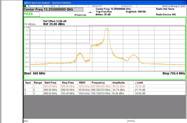
Band 12 1.4MHz/699.7/Low 16QAM 1@5
