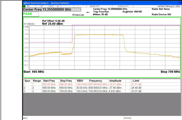
Band 12 5MHz/701.5/Low QPSK 25@0
