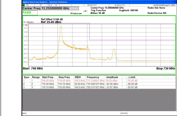
Band 12 5MHz/713.5/High QPSK 1@0
