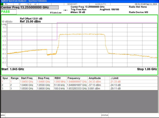
Band 2 5MHz/1852.5/Low 16QAM 25@0
