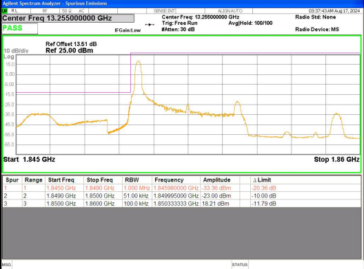
Band 2 5MHz/1852.5/Low 16QAM 1@0
