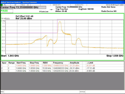
Band 2 1.4MHz/1850.7/Low 16QAM 1@C
