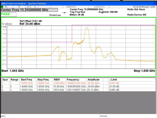
Band 2 1.4MHz/1850.7/Low QPSK 1@5
