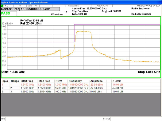
Band 2 1.4MHz/1850.7/Low 16QAM 6@C
