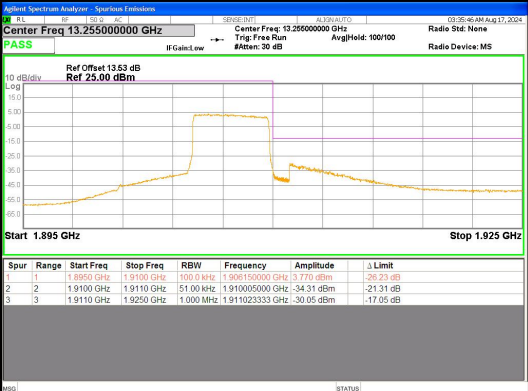
Band 2 5MHz/1907.5/High 16QAM 25@0
