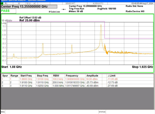
Band 2 20MHz/1900.0/High QPSK 1@99
