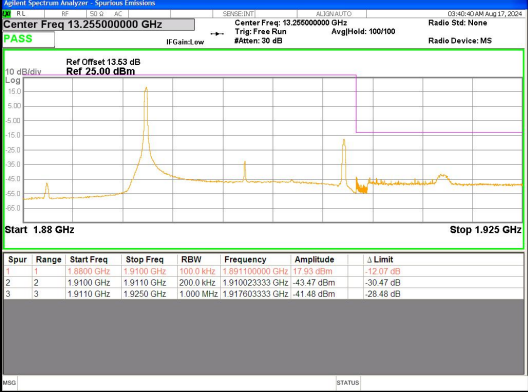
Band 2 20MHz/1900.0/High 16QAM 1@0
