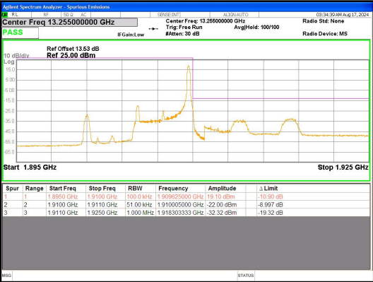
Band 2 5MHz/1907.5/High QPSK 1@24
