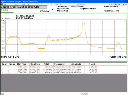
Band 2 5MHz/1852.5/Low QPSK 1@24
