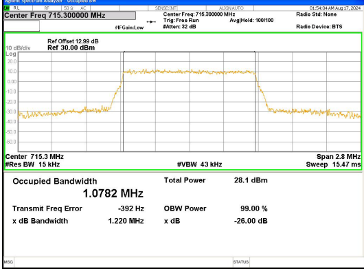
Band 12 1.4MHz/715.3/High 16QAM 6@0
