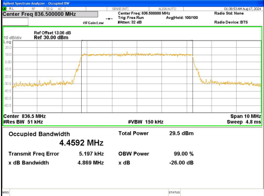
Band 5 5MHz/836.5/Mid 16QAM 25@0
