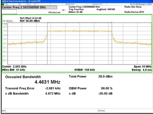
Band 7 5MHz/2502.5/Low 16QAM 25@0
