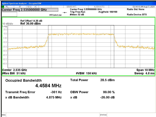
Band 7 5MHz/2535.0/Mid 16QAM 25@0
