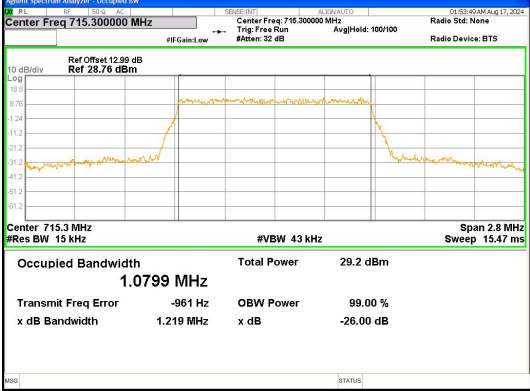
Band 12 1.4MHz/715.3/High QPSK 6@0
