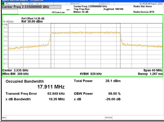
Band 7 20MHz/2535.0/Mid 16QAM 100@0
