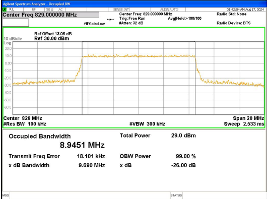
Band 5 10MHz/829.0/Low 16QAM 50@0
