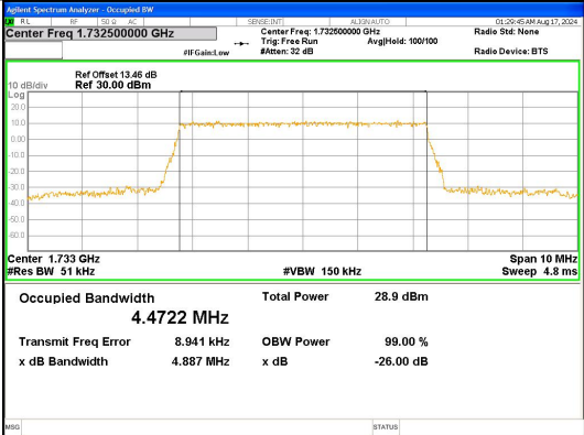
Band 4 5MHz/1732.5/Mid 16QAM 25@0
