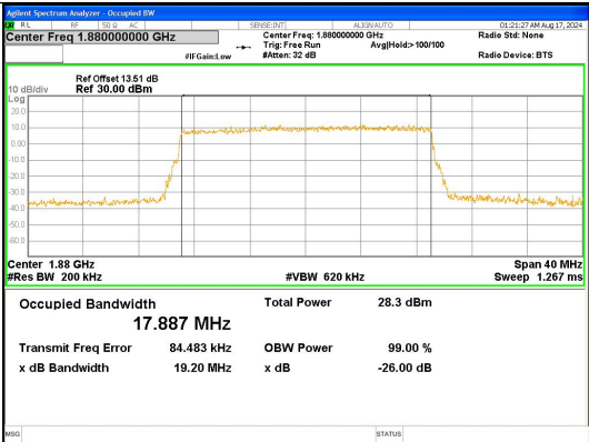
Band 2 20MHz/1880.0/Mid 16QAM 100@0
