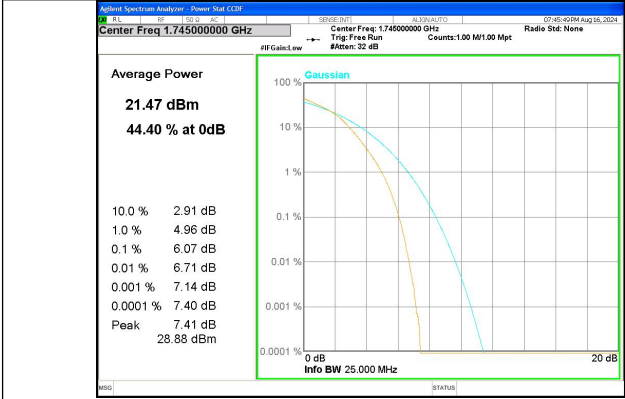
Band 66 20MHz/1745.0/Mid 16QAM 100@@
