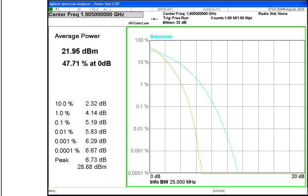
Band 25 20MHz/1905.0/High 16QAM 100@@
