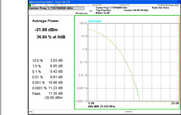
Band 66 1.4MHz/1710.7/Low 16QAM 6@@
