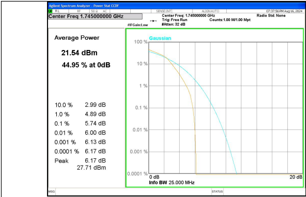
Band 66 1.4MHz/1745.0/Mid 16QAM 6@@
