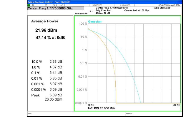
Band 66 5MHz/1777.5/High QPSK 25@@
