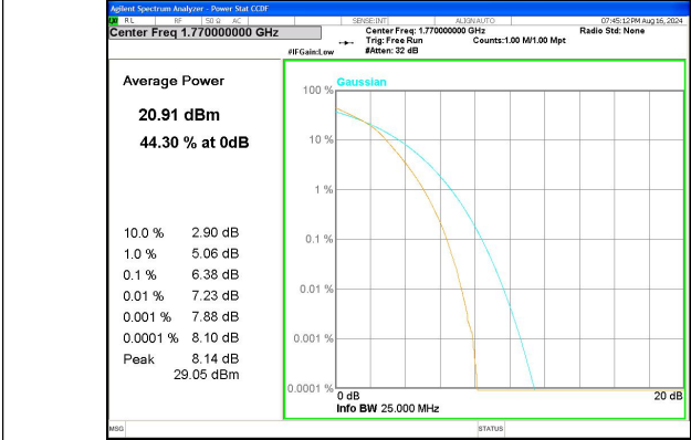
Band 66 20MHz/1770.0/High 16QAM 100@@
