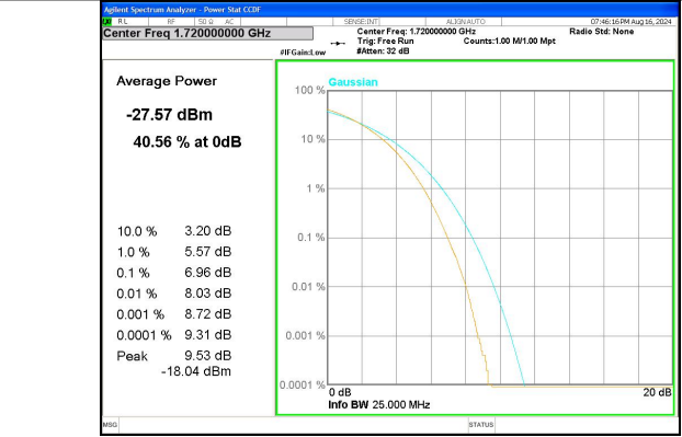
Band 66 20MHz/1720.0/Low QPSK 100@@
