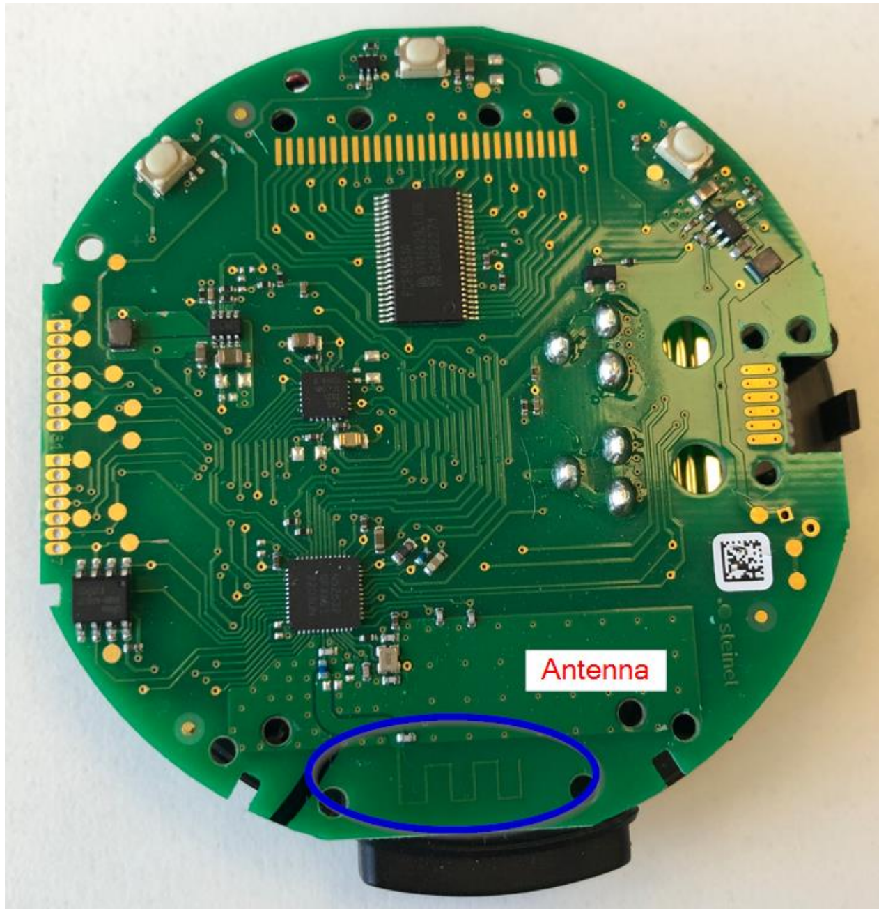
Inside with Antenna location
