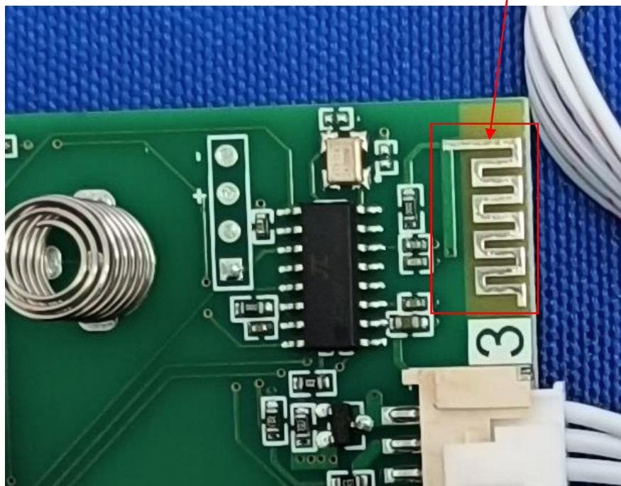
PCB Antenna
