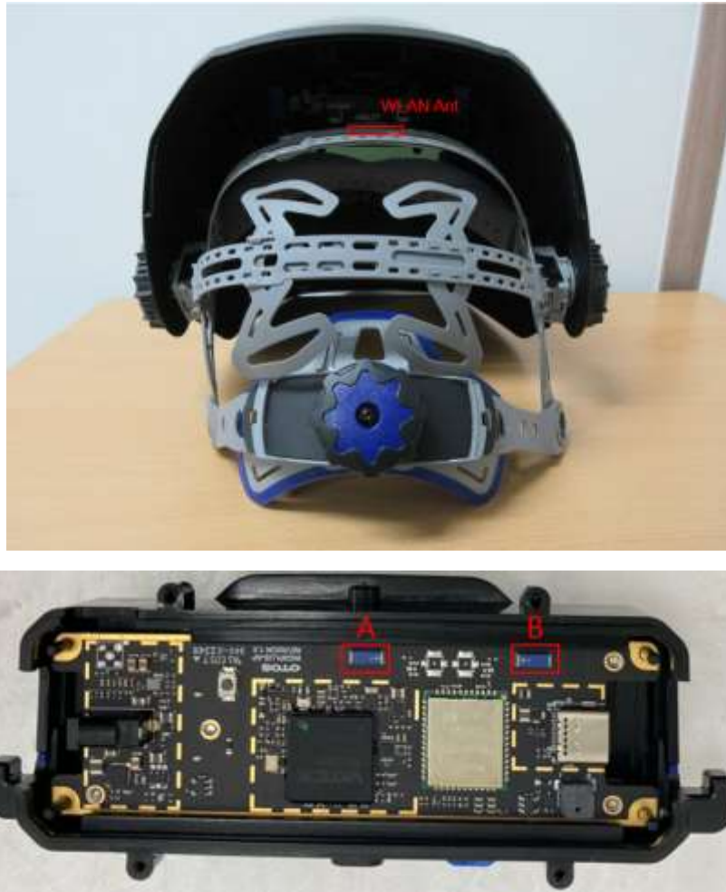
Figure F-1 WLAN Antenna Location
