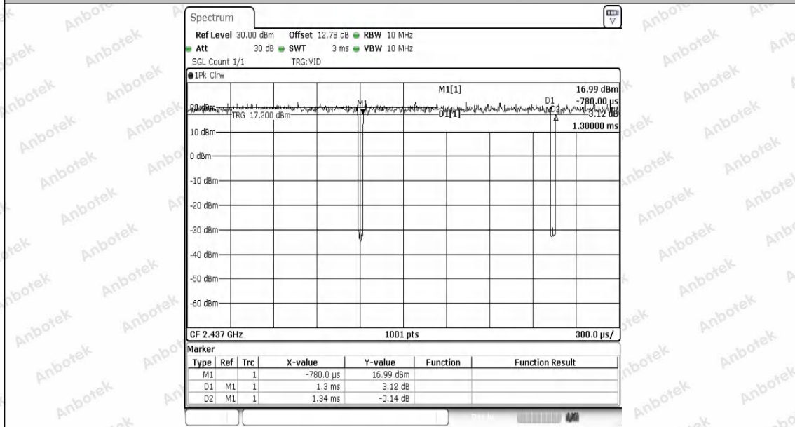
NTNV-11N20SISO-Ant1-2437
