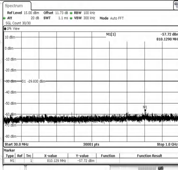
11N20SISO-Ant1-2462-30~1000-PASS
