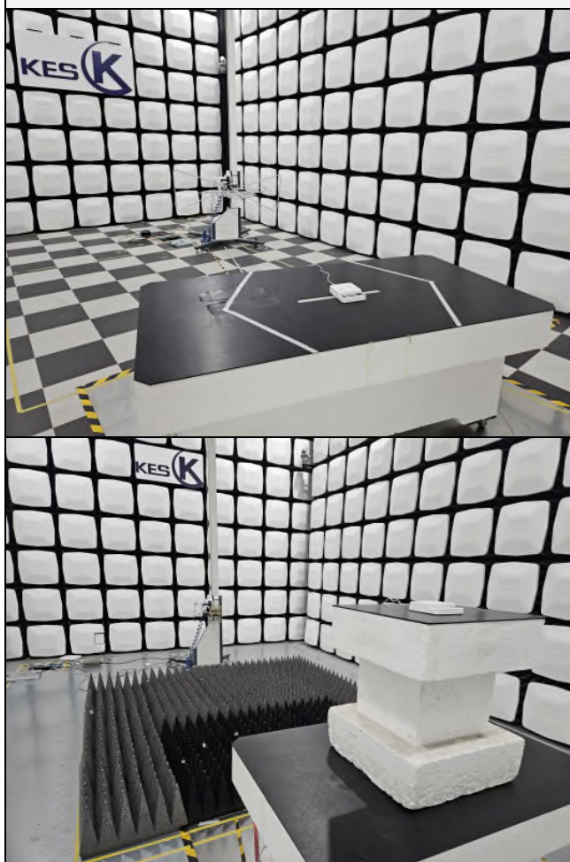
Radiated test
