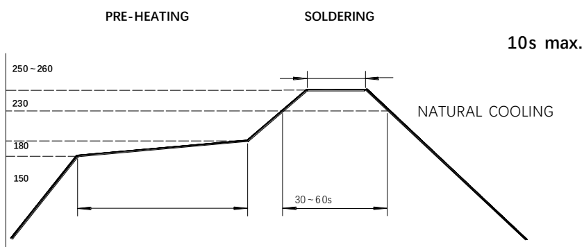
Reflow Soldering
