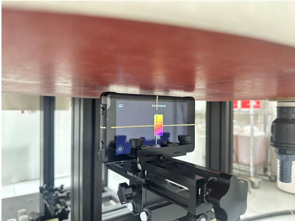
Description: Body Bottom Position with 5mm gap
