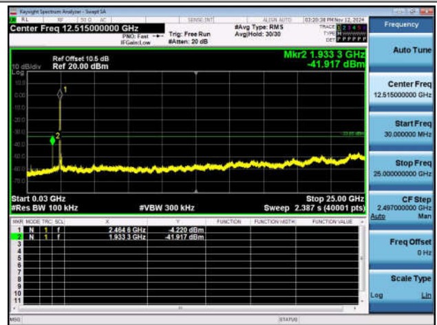
11N40SISO-Ant1-2452-30~25000-PASS
