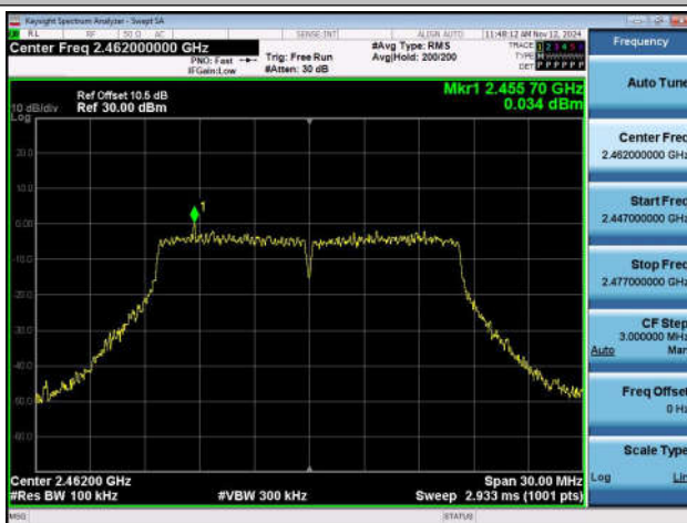
11G-Ant1-2462-0~Reference-PASS
