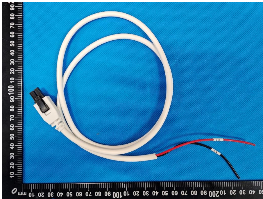
Accessory-Interface Cable (Blue Comprehensive)
