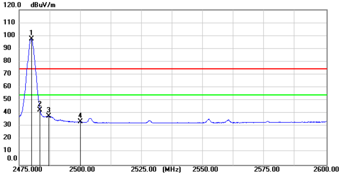
BLE_2M_TX_CH_39_Horizontal_Average
