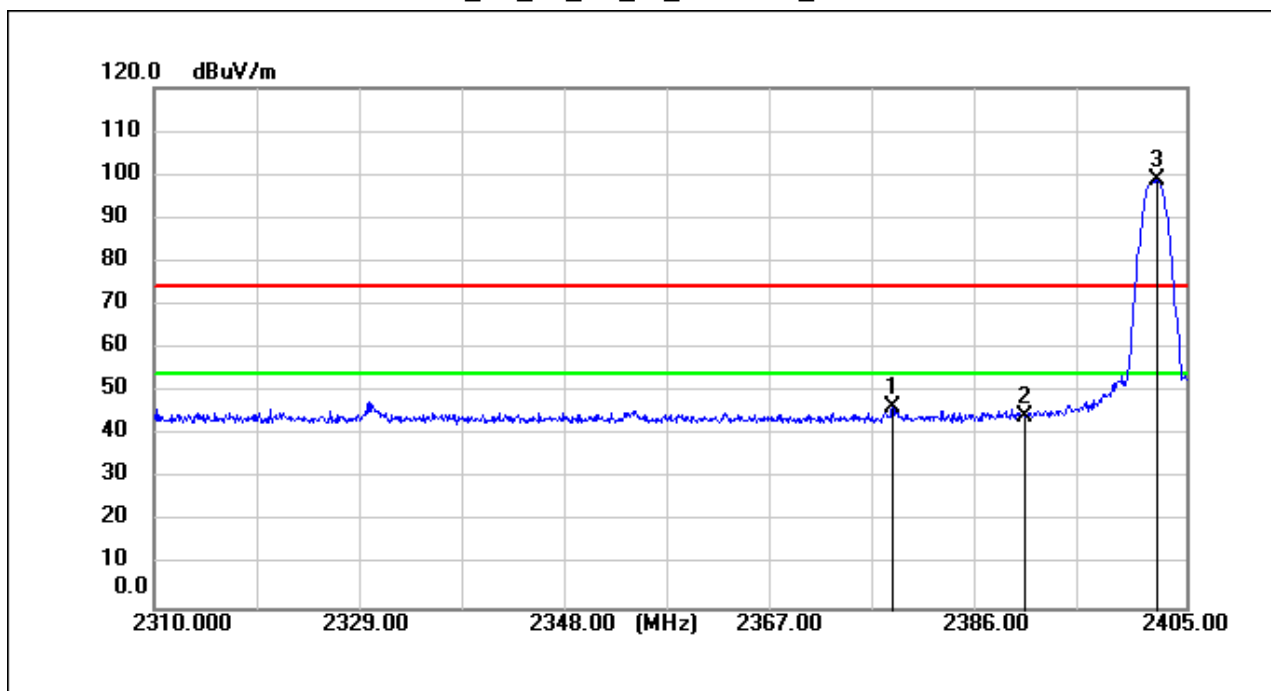
BLE_1M_TX_CH_00_Horizontal_Peak
