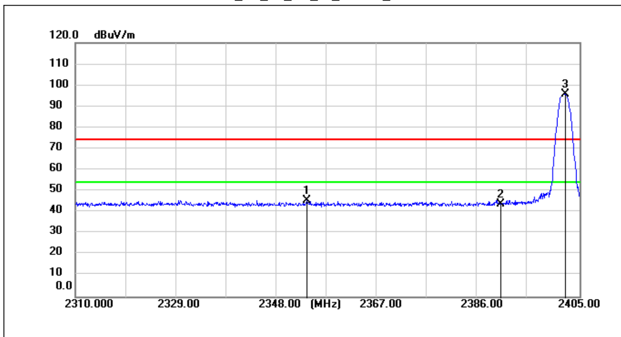
BLE_1M_TX_CH_00_Vertical_Peak
