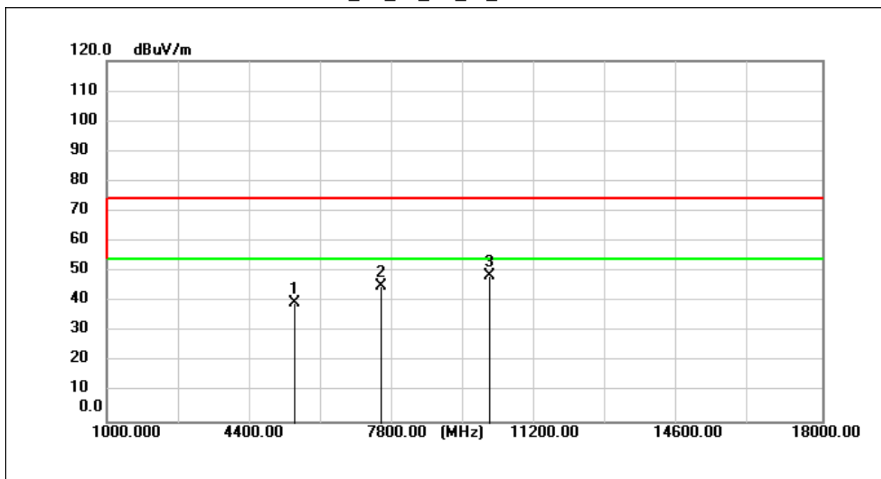
BLE_2M_TX_CH_19_Horizontal
