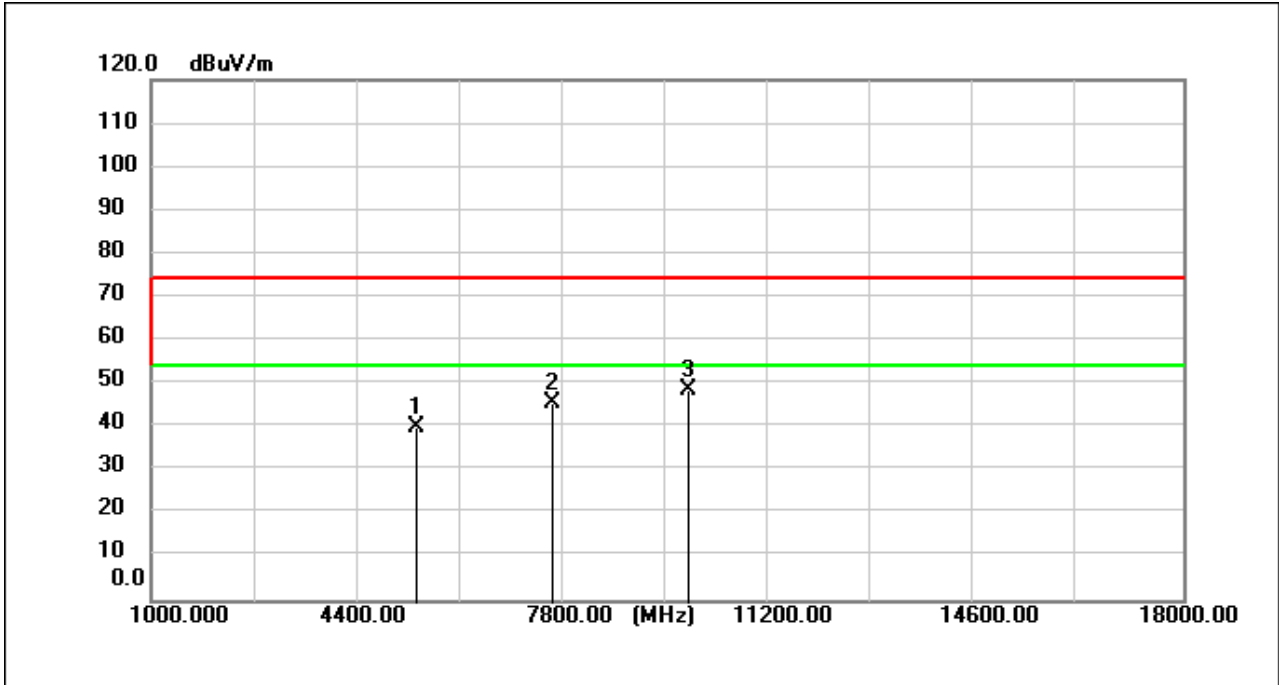
BLE_2M_TX_CH_19_Verical
