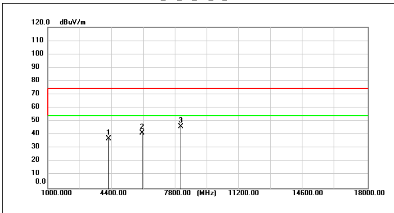
BLE_1M_TX_CH_39_Verical
