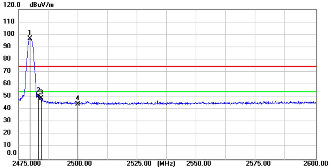
BLE_1M_TX_CH_39_Verical
