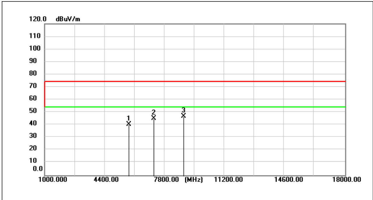
BLE_1M_TX_CH_19_Verical
