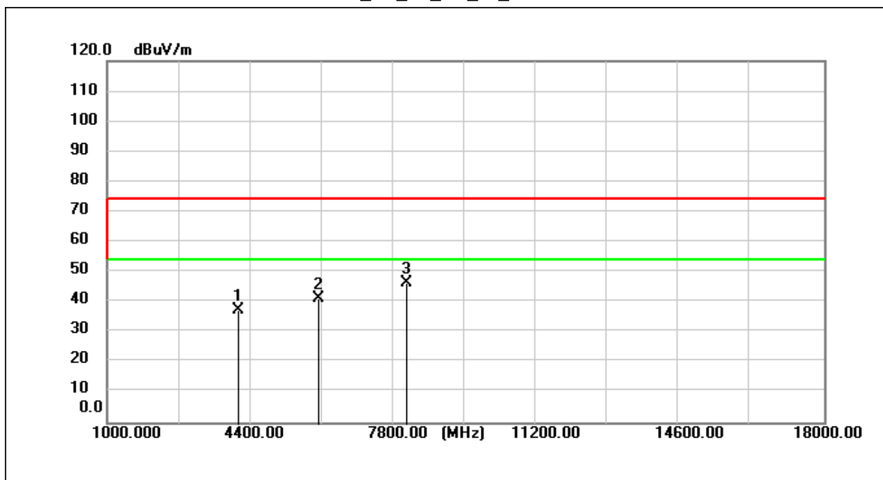
BLE_1M_TX_CH_00_Verical
