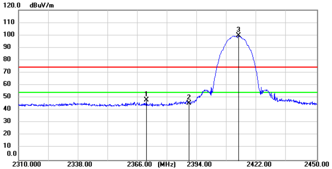
11b_TX_CH_01_Vertical_Peak
