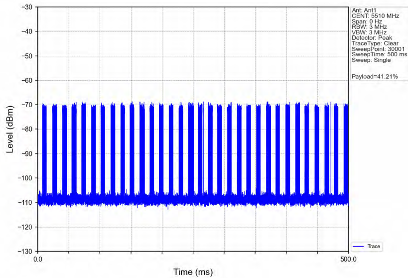
Channel Loading (Payload) 802.11ax(HEW40) 2C 5510MHz
