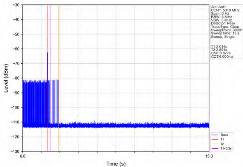
Channel Move Time and Closing Transmission Time_802.11ax(HEW40)_2A_5310MHz
