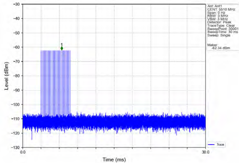
Signal Calibration 802.11ax(HEW40) 2C 5510MHz RadarType3 Trial0
