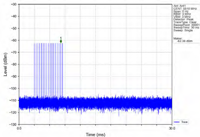
Signal Calibration 802.11ax(HEW40) 2C 5510MHz RadarType3 Trial0
