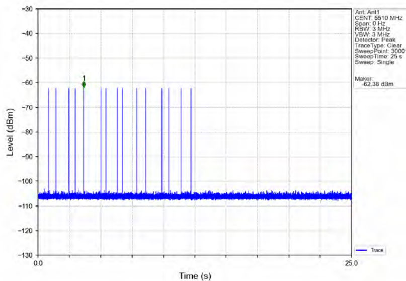
Signal Calibration 802.11ax(HEW40) 2C 5510MHz RadarType5 Trial0
