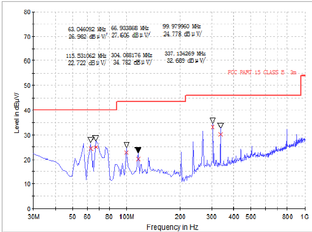
EMI Sweep-3M(30-1G)
