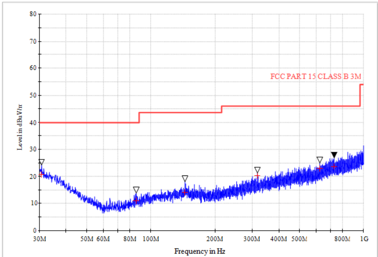
(Plot C: Test Antenna Vertical 30M - 1G)
