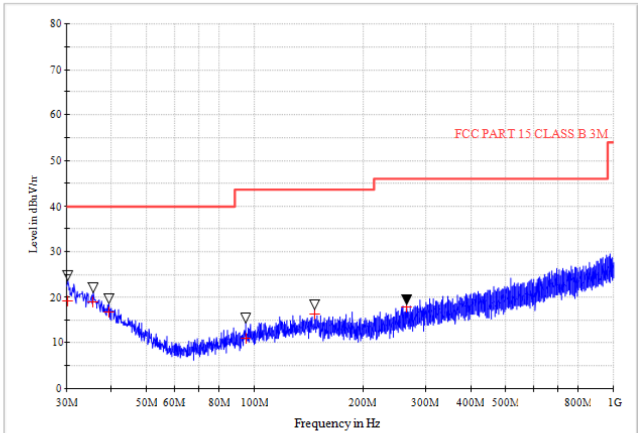
(Plot D: Test Antenna Horizontal 30M - 1G)
