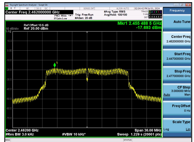
11G-Ant1-2462-PASS
