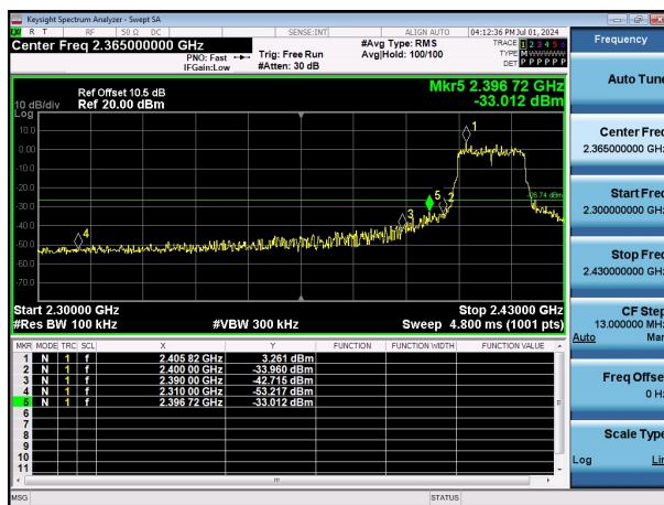
11G-Ant1-2412-PASS
