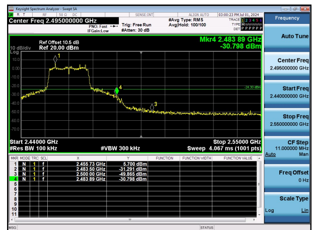
11N20SISO-Ant1-2462-PASS
