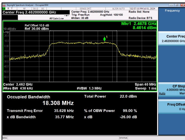
11N20SISO-Ant1-2462
