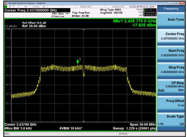
11N20SISO-Ant1-2437-PASS
