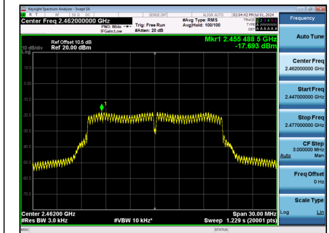
11G-Ant1-2462-PASS
