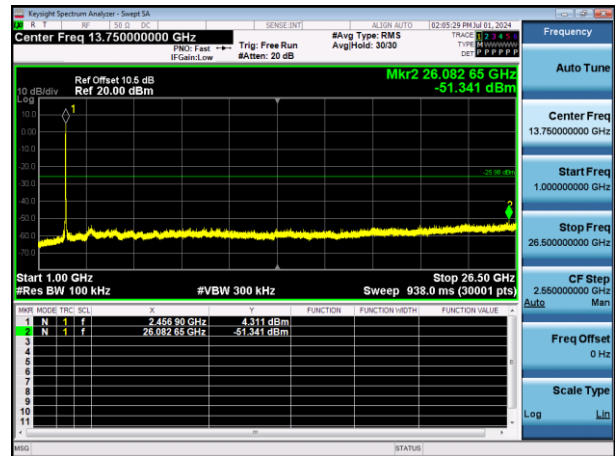
11G-Ant1-2462-1000~26500-PASS
