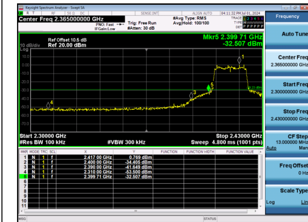
11N20SISO-Ant1-2412-PASS
