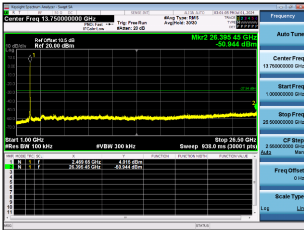
11N20SISO-Ant1-2462-1000~26500-PASS
