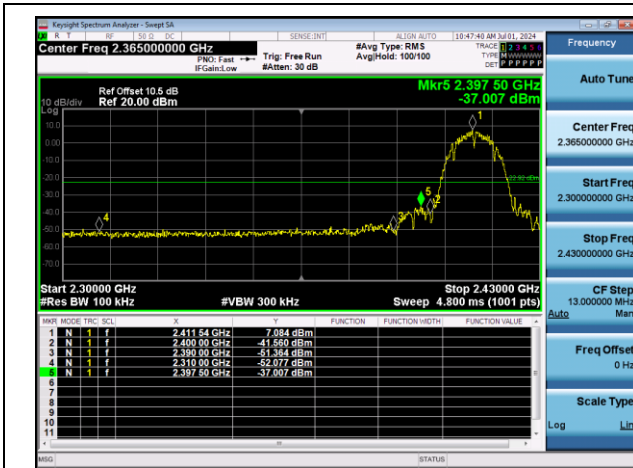
11B-Ant1-2412-PASS
