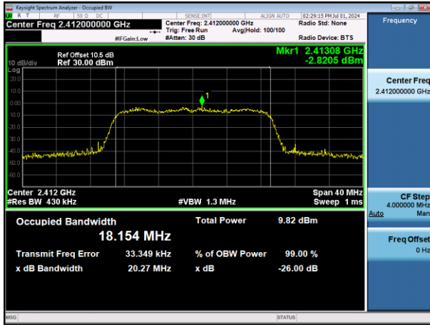
11N20SISO-Ant1-2412
