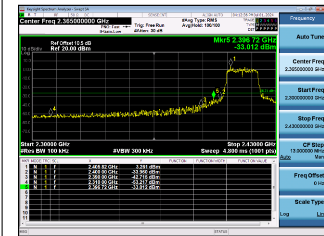
11G-Ant1-2412-PASS
