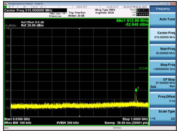
11N20SISO-Ant1-2412-30~1000-PASS
