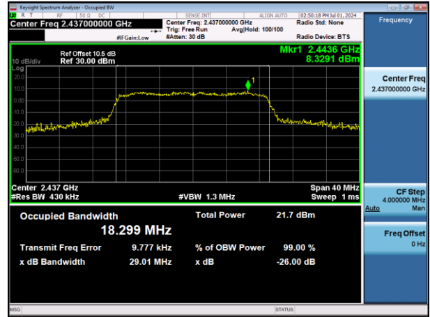
11N20SISO-Ant1-2437
