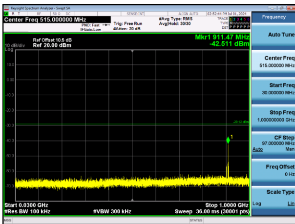
11N20SISO-Ant1-2437-30~1000-PASS
