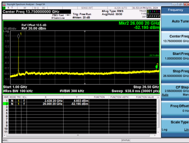
11G-Ant1-2437-1000~26500-PASS
