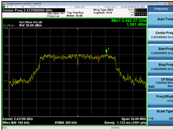
11G-Ant1-2437-0~Reference-PASS
