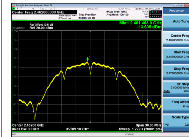
11B-Ant1-2462-PASS
