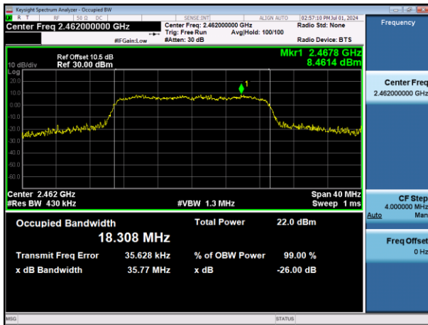
11N20SISO-Ant1-2462
