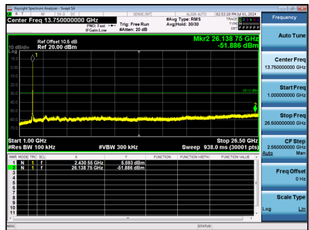
11N20SISO-Ant1-2437-1000~26500-PASS
