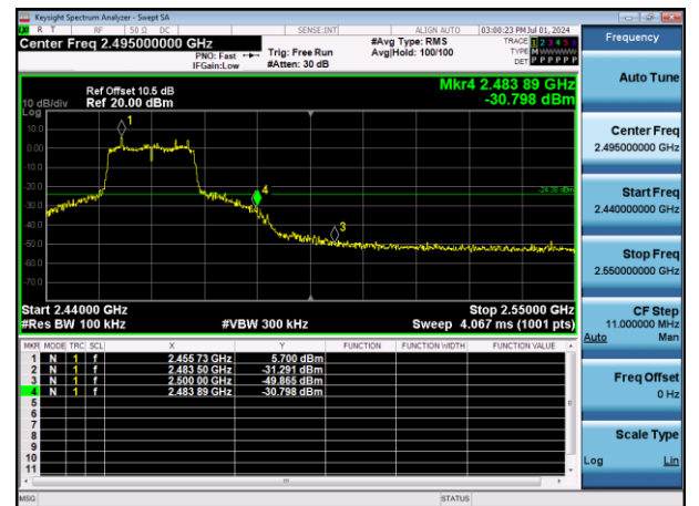
11N20SISO-Ant1-2462-PASS
