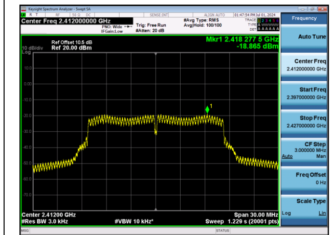
11G-Ant1-2412-PASS
