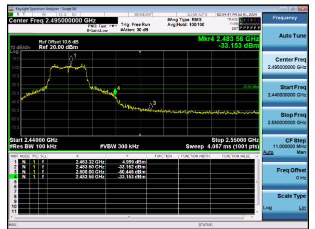
11G-Ant1-2462-PASS
