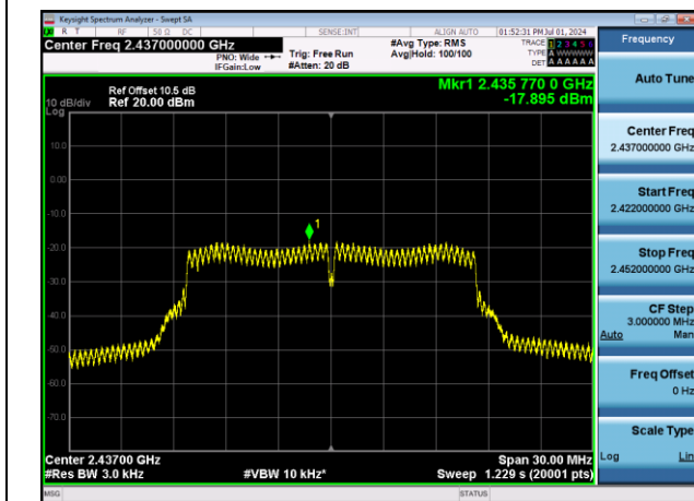
11G-Ant1-2437-PASS
