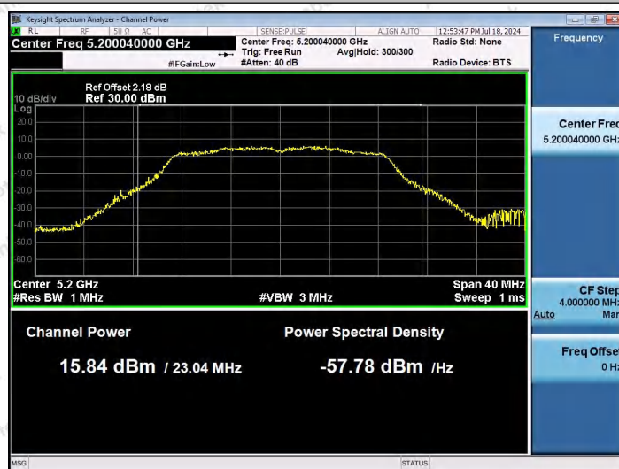
11AC20SISO-Ant1-5200-PASS
