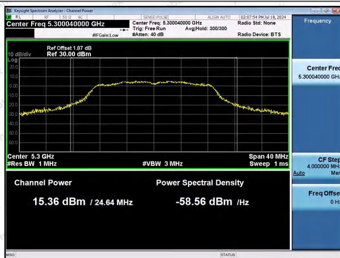
11AC20SISO-Ant1-5300-PASS
