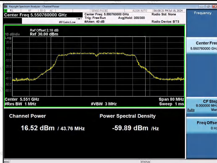
11AC40SISO-Ant1-5550-PASS
