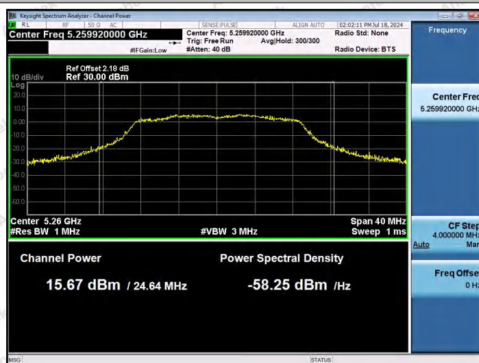
11AC20SISO-Ant1-5260-PASS
