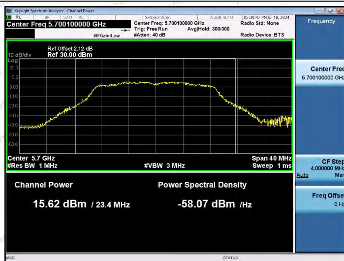
11N20SISO-Ant1-5700-PASS
