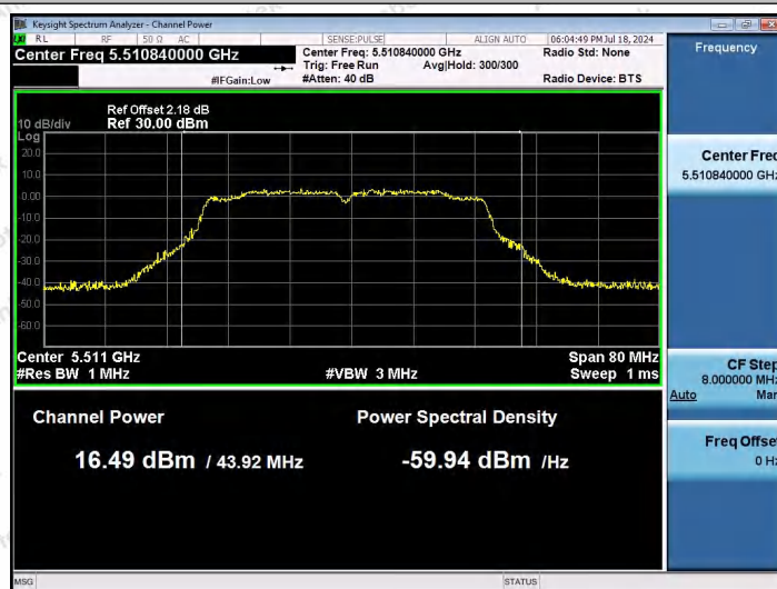
11AC40SISO-Ant1-5510-PASS
