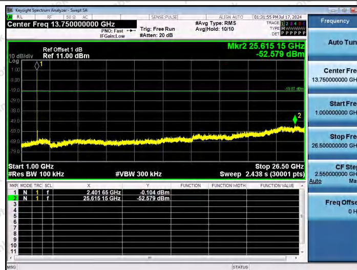
DH5-Ant1-2402-1000~26500-PASS
