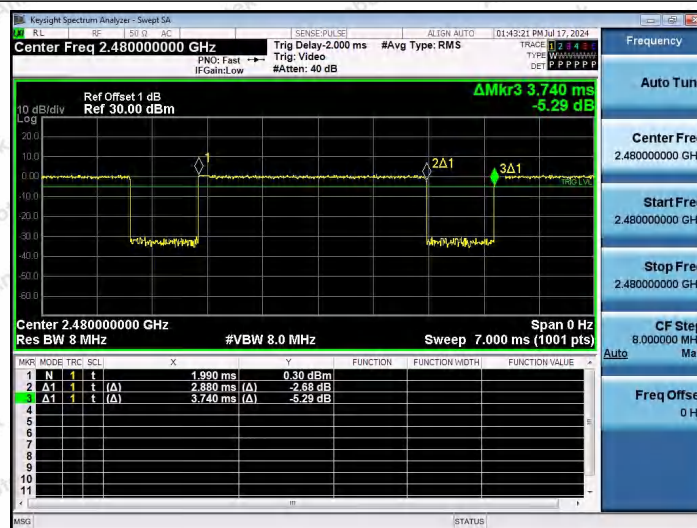
NTVN-3DH5-Ant1-2480
