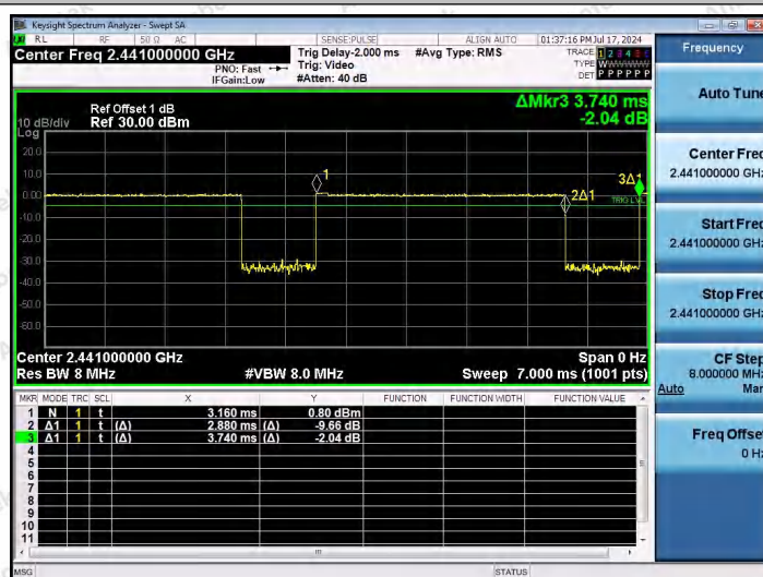
NTNV-2DH5-Ant1-2441
