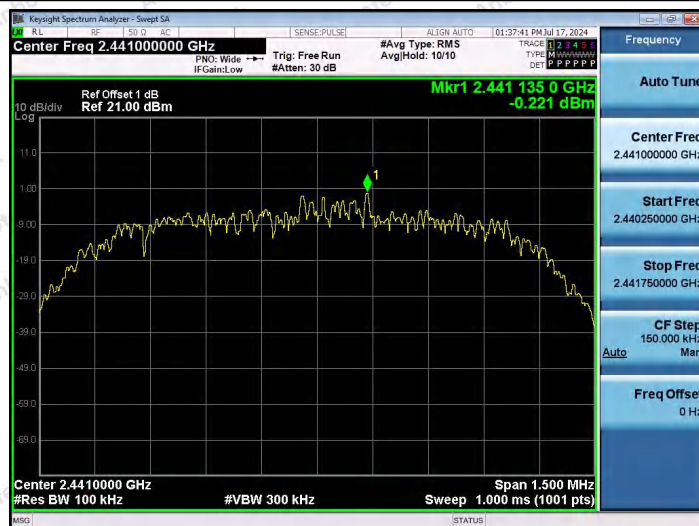
2DH5-Ant1-2441-0~Reference-PASS
