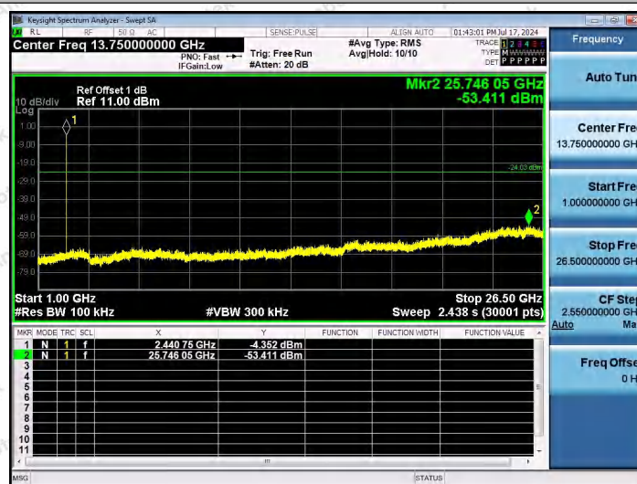
3DH5-Ant1-2441-1000~26500-PASS
