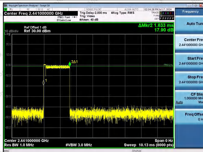
3DH3-Ant1-Hop-PASS
