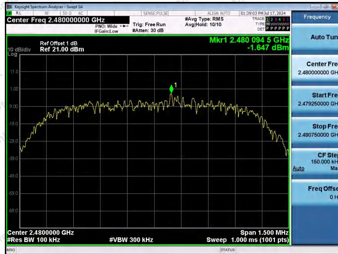
2DH5-Ant1-2480-0~Reference-PASS
