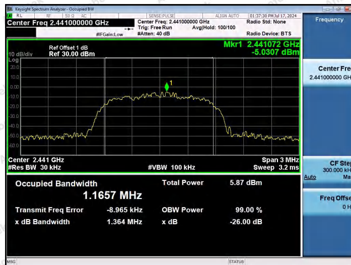
2DH5-Ant1-2441
