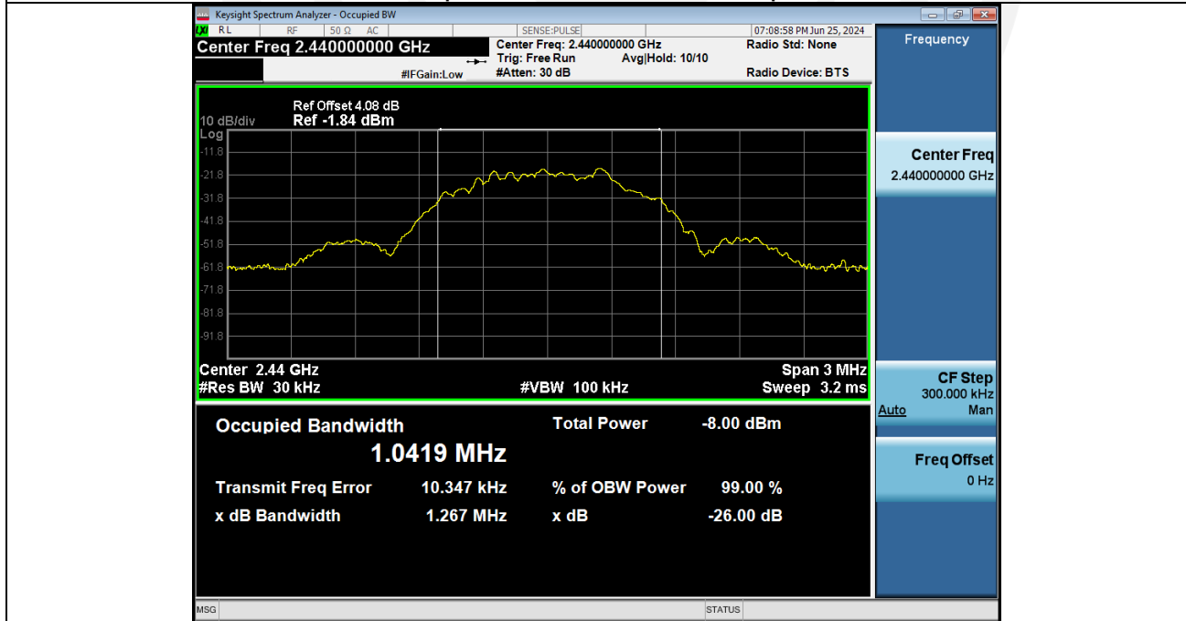
99% Occupied Bandwidth NVNT ANT1 1Mbps 2440
