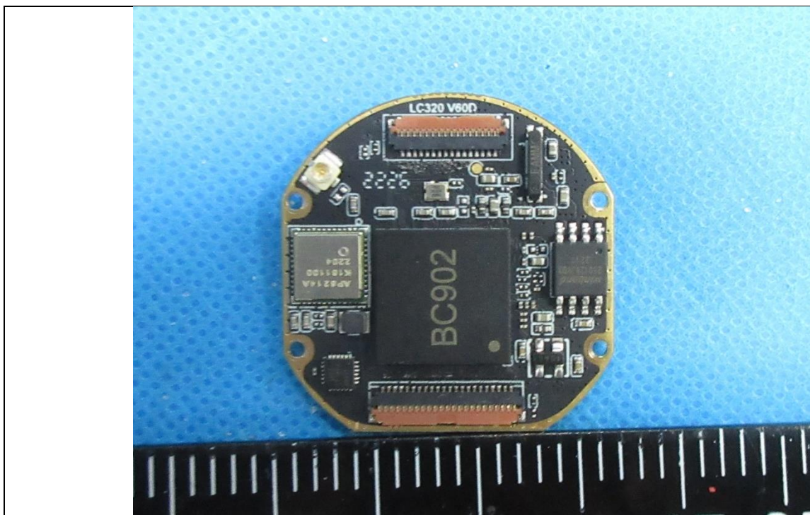
Details of: Internal view 10 (SUPER YOTER LRF 35mm)
