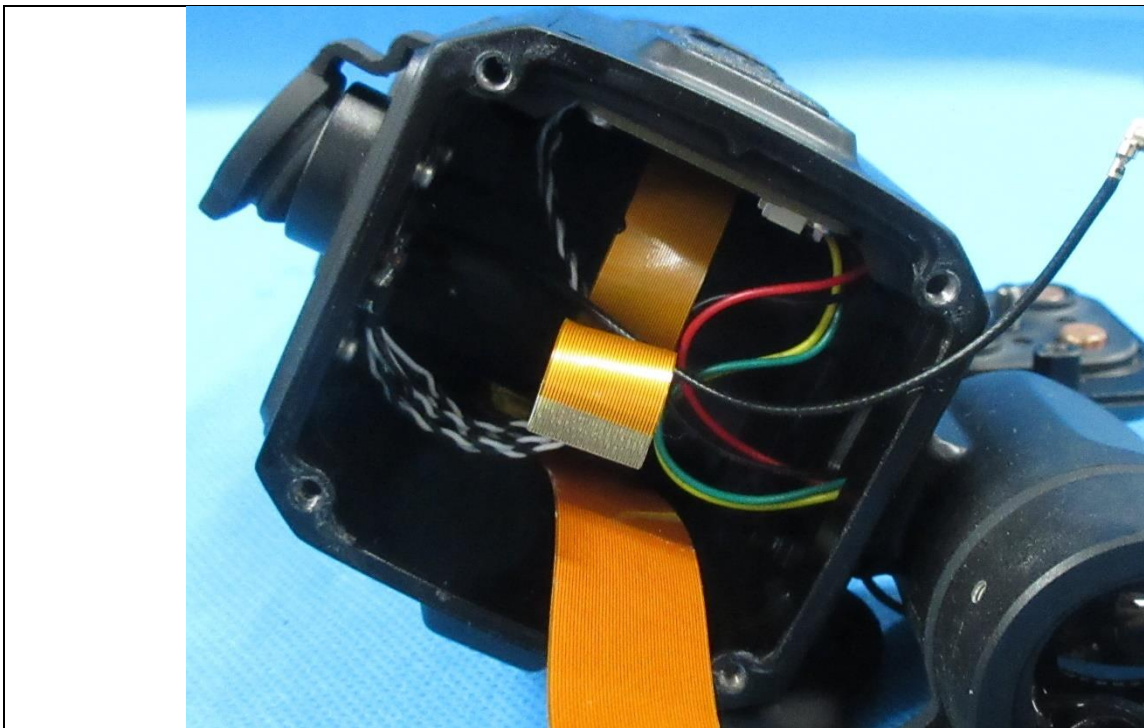
Details of: Internal view 7 (SUPER YOTER LRF 35mm)
