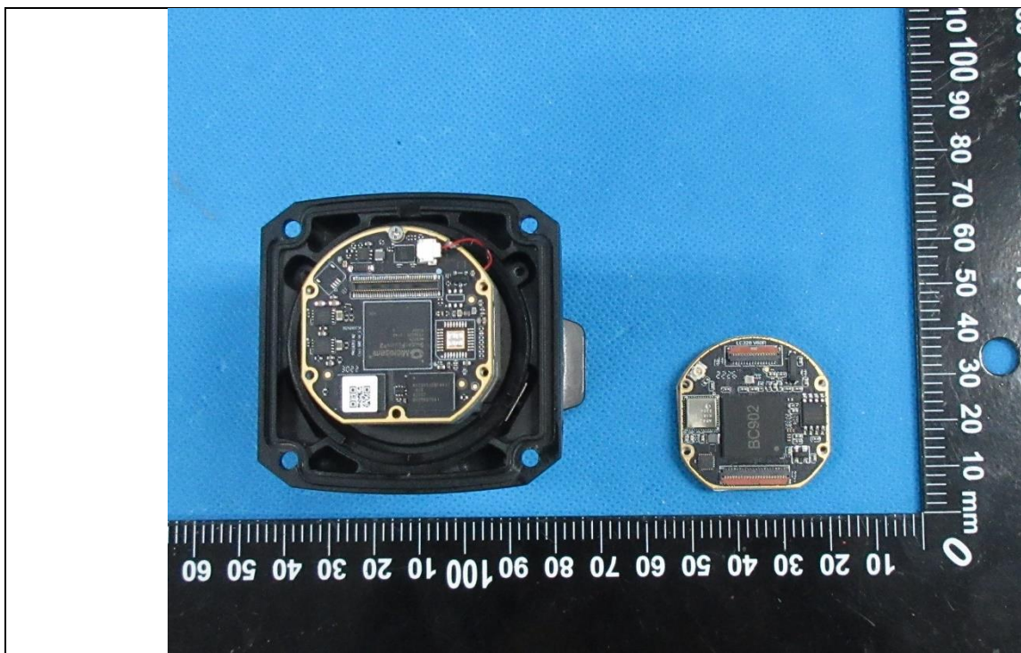
Details of: Internal view 8 (SUPER YOTER LRF 35mm)
