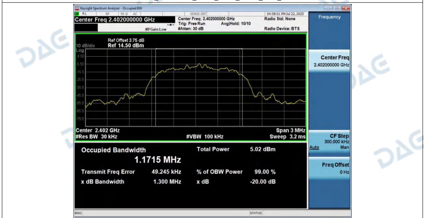
-20dB_Bandwidth_NVNT_ANT1_3-DH5_2402_00
