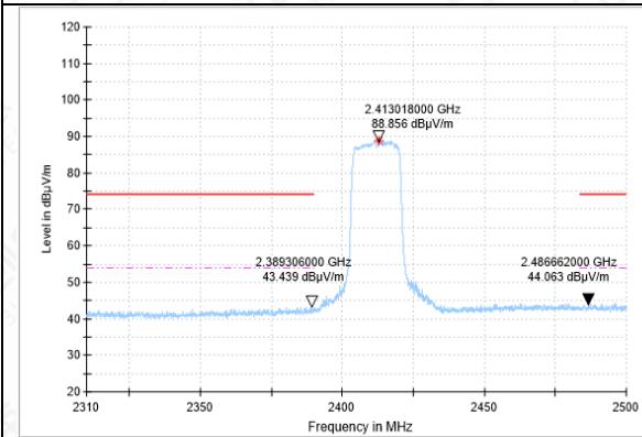
Bandedge-11G-CH1-AV
