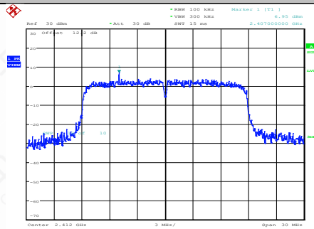
11N20SISO-Ant1-2412-0~Reference-PASS
