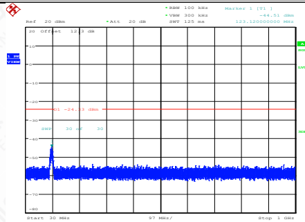
11N20SISO-Ant1-2437-30~1000-PASS
