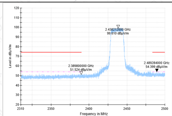
Bandedge-11G-CH6-PK
