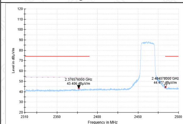
Bandedge-11G-CH11-AV
