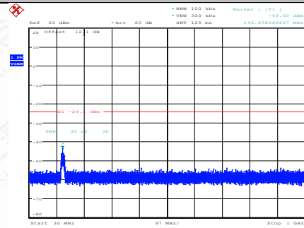
11N20SISO-Ant1-2462-30~1000-PASS
