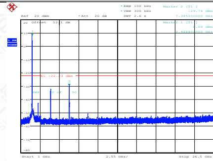
11G-Ant1-2462-1000~26500-PASS
