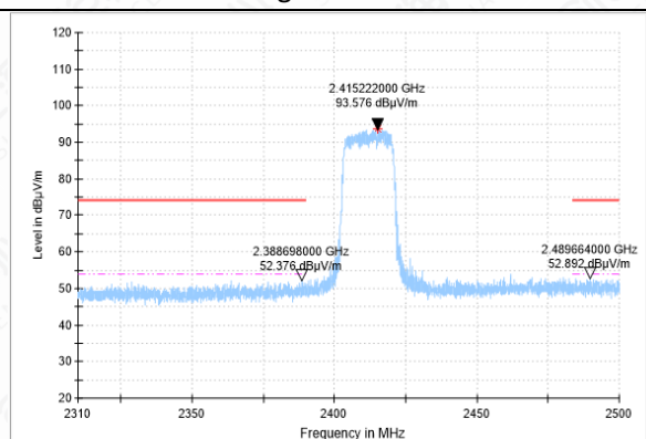
Bandedge-11N-CH1-PK
