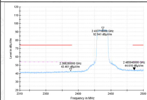
Bandedge-11G-CH6-AV
