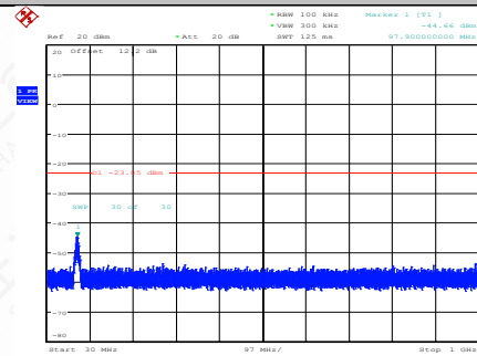
11N20SISO-Ant1-2412-30~1000-PASS
