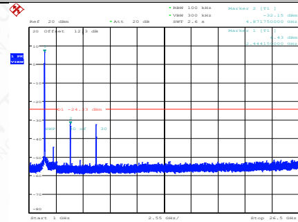
11N20SISO-Ant1-2437-1000~26500-PASS
