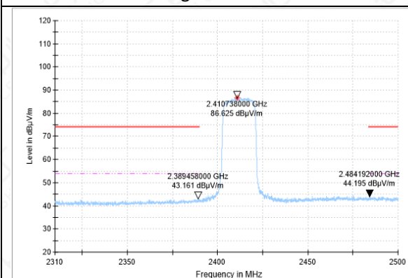
Bandedge-11N-CH1-AV
