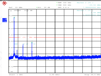
11N20SISO-Ant1-2462-1000~26500-PASS
