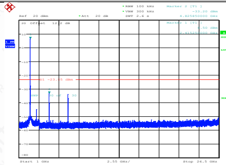
11N20SISO-Ant1-2412-1000~26500-PASS
