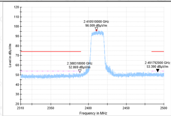
Bandedge-11G-CH1-PK
