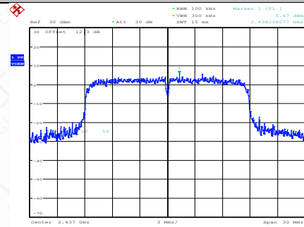
11N20SISO-Ant1-2437-0~Reference-PASS
