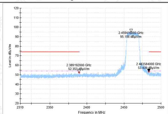
Bandedge-11G-CH11-PK
