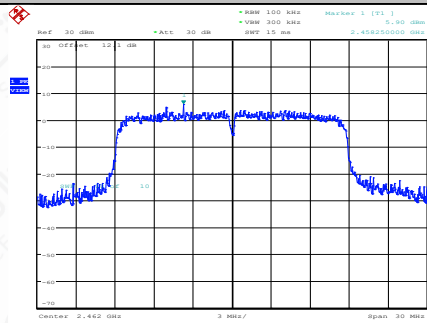
11N20SISO-Ant1-2462-0~Reference-PASS
