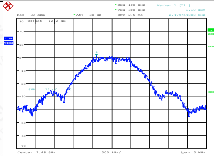
BLE_125K-Ant1-2480-0~Reference-PASS
