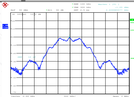
BLE_500K-Ant1-2440-0~Reference-PASS
