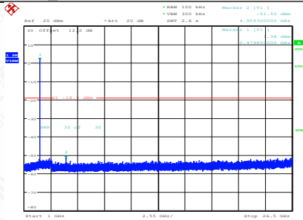
BLE_125K-Ant1-2480-1000~26500-PASS
