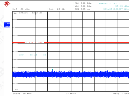
BLE_125K-Ant1-2480-30~1000-PASS
