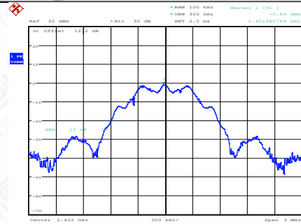
BLE_500K-Ant1-2402-0~Reference-PASS
