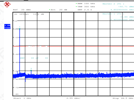
BLE_500K-Ant1-2402-1000~26500-PASS
