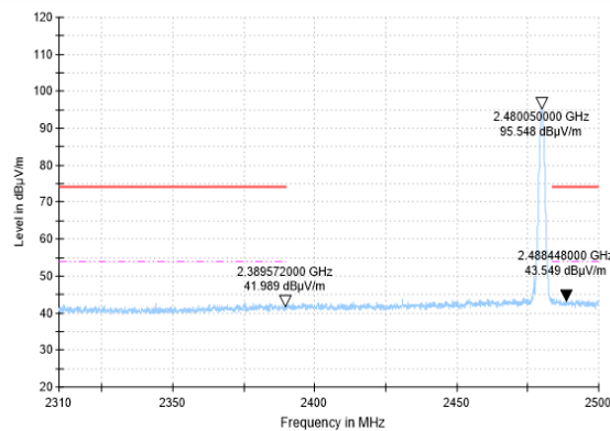
Bandedge-Coded S=8-CH39-AV
