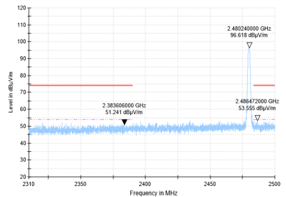
Bandedge-Coded S=8-CH39-PK
