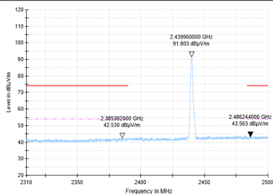
Bandedge-Coded S=8-CH39-AV
