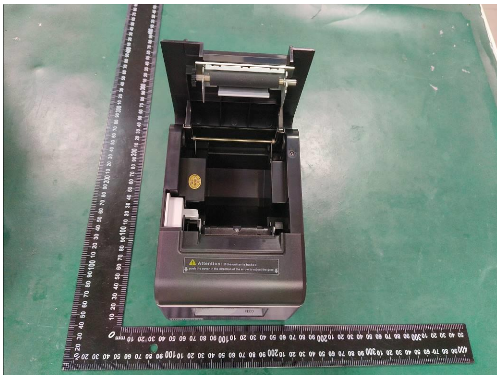
Internal Photo FCC ID: 2BHCJ-WPC58W
