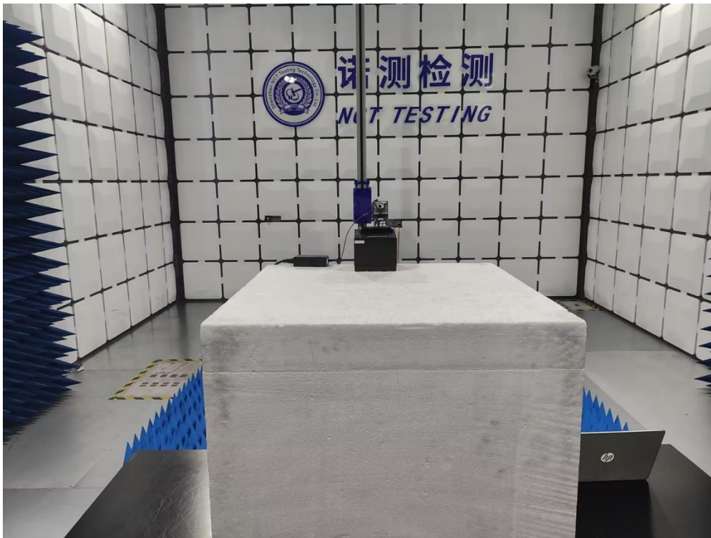
Setup Photo FCC ID: 2BHCJ-WPA1W
