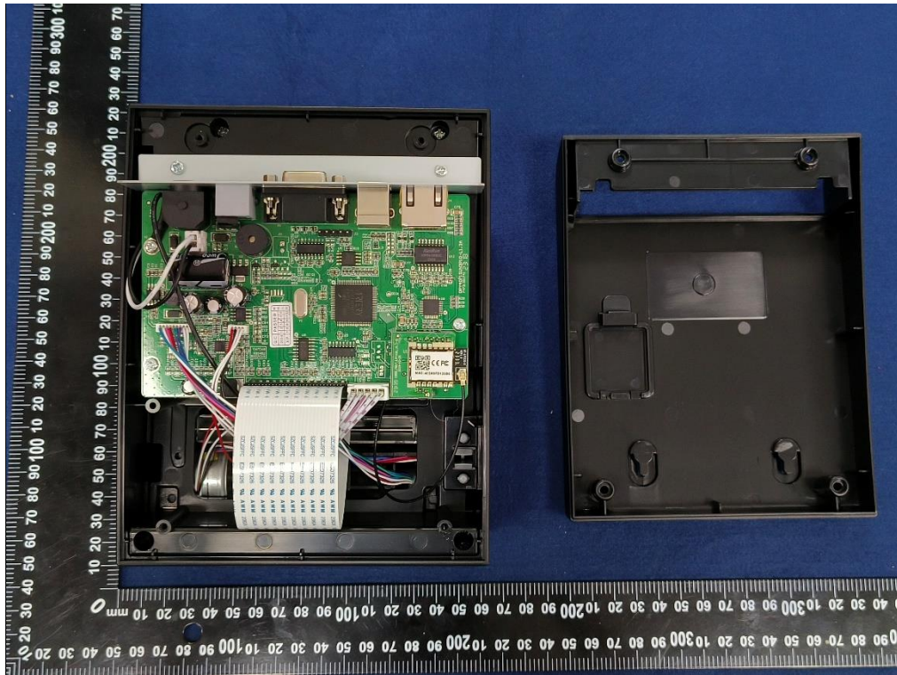
Internal Photo FCC ID: 2BHCJ-WPA1W
