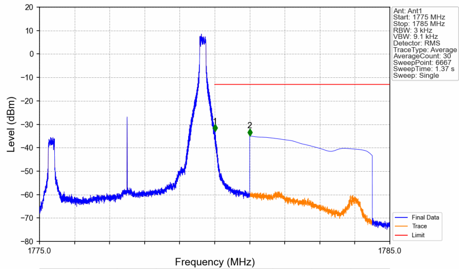
Band66 5MHz 16QAM HCH 1777.5MHz RB 1 24 NTNV
