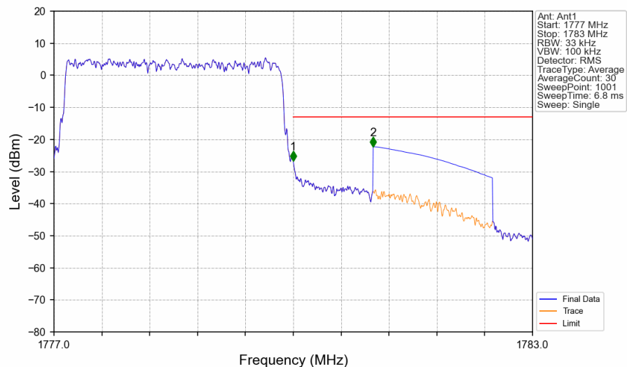
Band66 3MHz 16QAM HCH 1778.5MHz RB 15 0 NTNV
