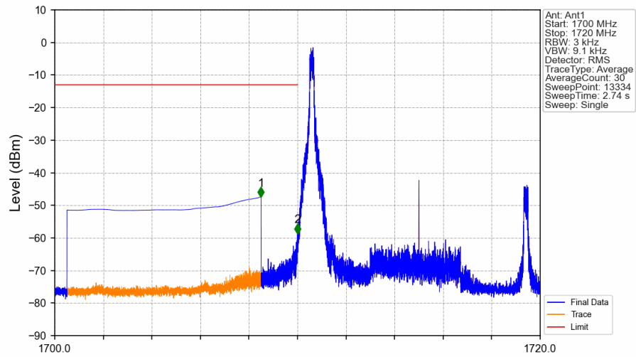
Band66_10MHz_QPSK_LCH_1715MHz_RB_1_0_NTNV
