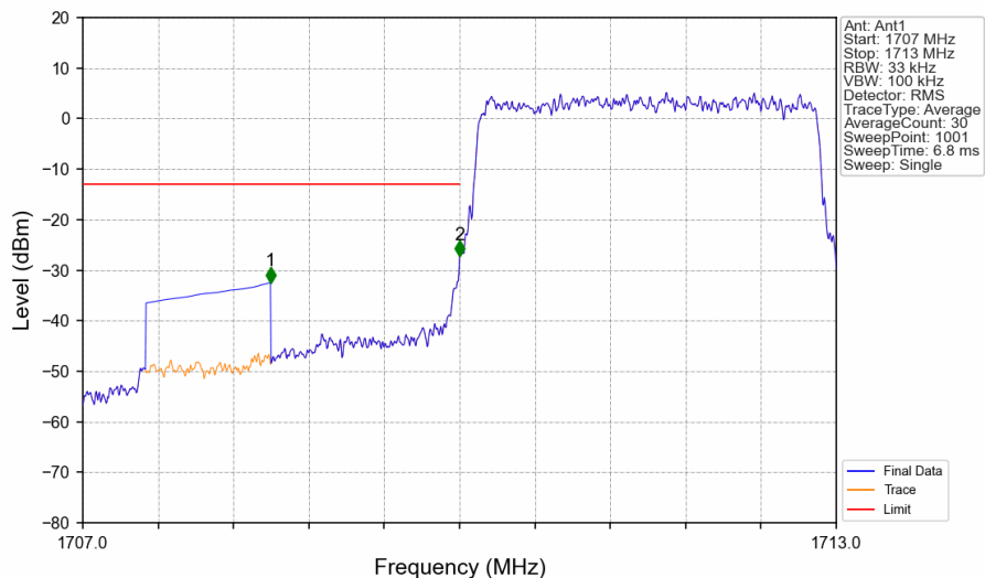
Band66_3MHz_QPSK_LCH_1711.5MHz_RB_15_0_NTNV
