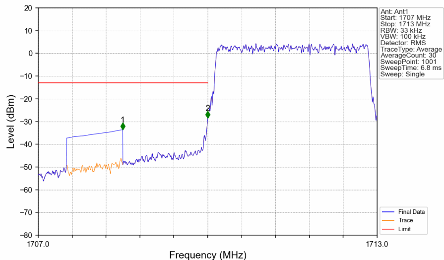
Band66_3MHz_16QAM_LCH_1711.5MHz_RB_15_0_NTNV
