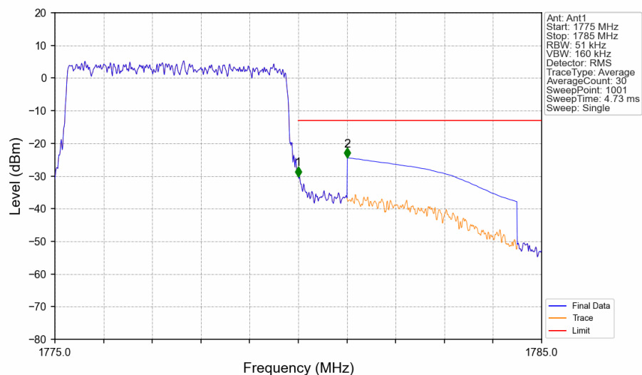
Band66 5MHz 16QAM HCH 1777.5MHz RB 25 0 NTNV
