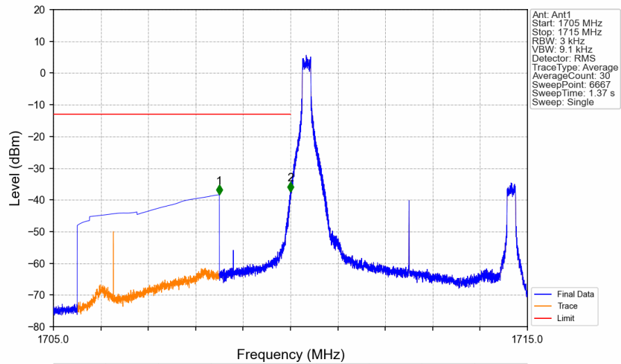
Band66_5MHz_16QAM_LCH_1712.5MHz_RB_1_0_NTNV
