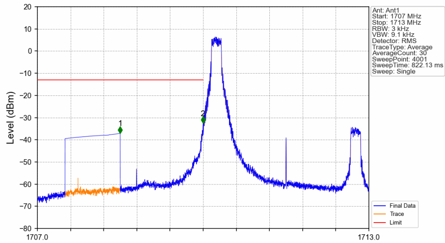
Band66_3MHz_QPSK_LCH_1711.5MHz_RB_1_0_NTNV
