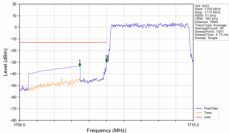
Band66_5MHz_16QAM_LCH_1712.5MHz_RB_25_0_NTNV
