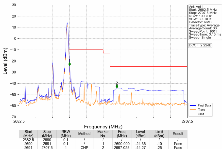
Band41 5MHz 16QAM HCH 2687.5MHz RB 1 24 NTNV
