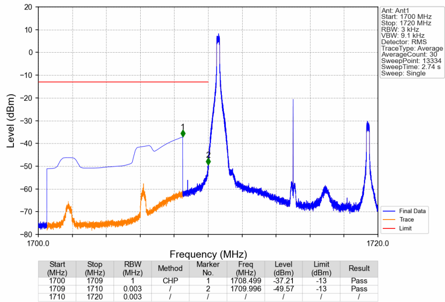
Band4_10MHz_QPSK_LCH_1715MHz_RB_1_0_NTNV
