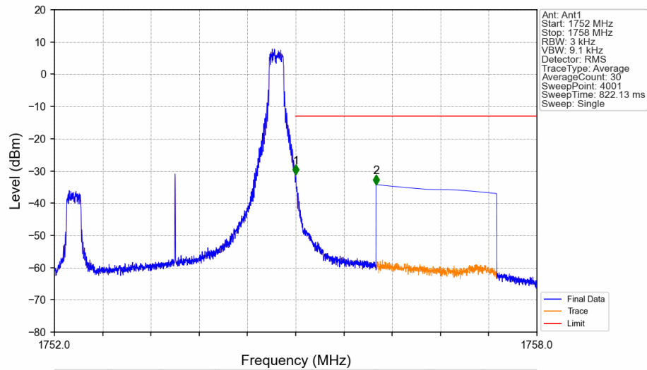
Band4 3MHz QPSK HCH 1753.5MHz RB 1 14 NTV
