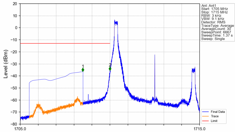
Band4_5MHz_QPSK_LCH_1712.5MHz_RB_1_0_NTNV
