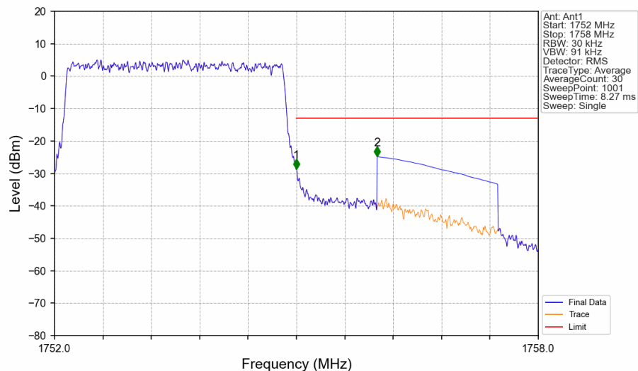
Band4 3MHz QPSK HCH 1753.5MHz RB 15 0 NTV
