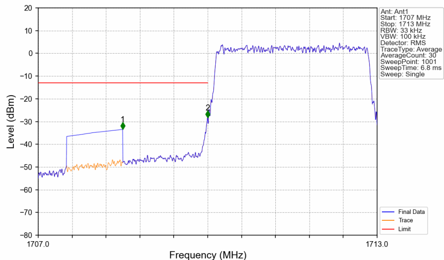
Band4 3MHz 16QAM LCH 1711.5MHz RB 15 0 NTNV
