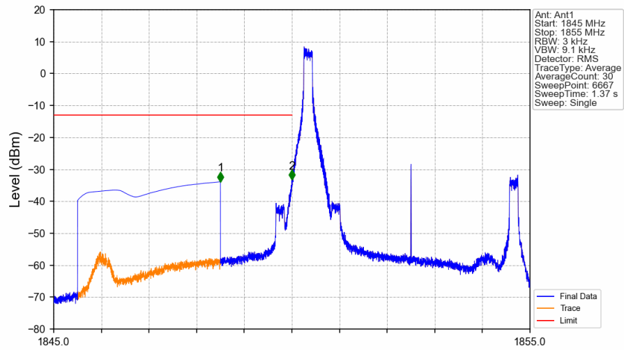
Band2_5MHz_QPSK_LCH_1852.5MHz_RB_1_0_NTNV
