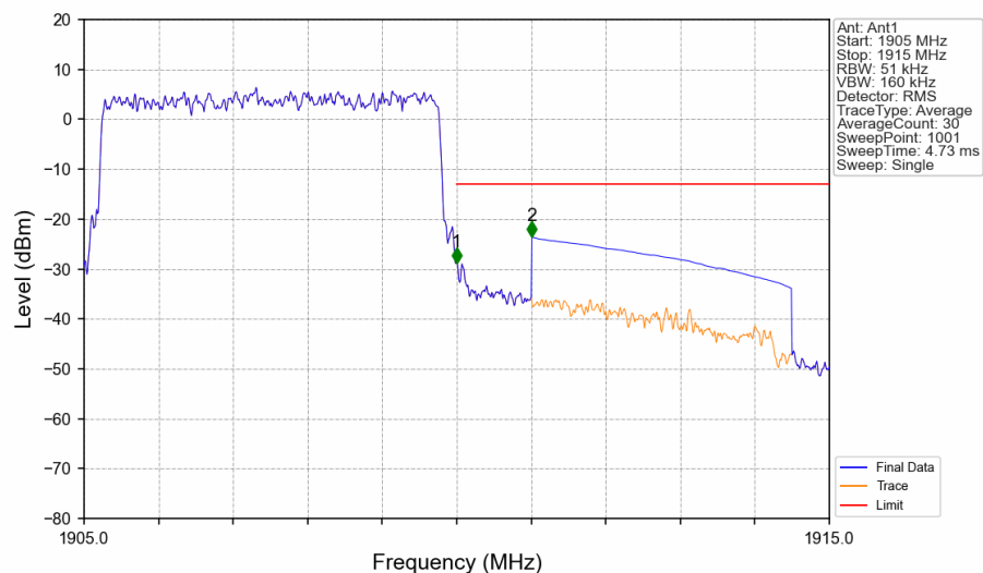
Band2_5MHz_QPSK_HCH_1907.5MHz_RB_25_0_NTNV
