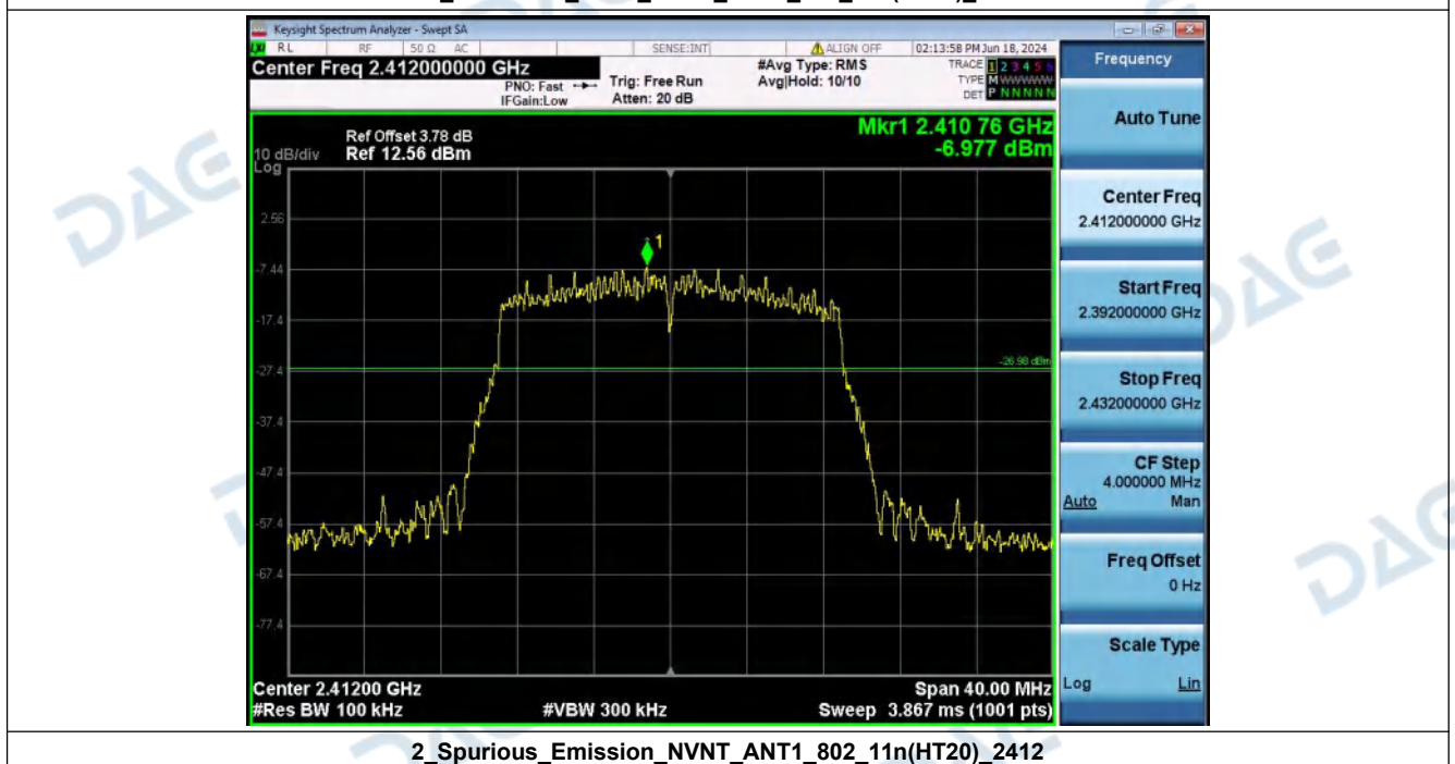
1_Reference_Level_NVNT_ANT1_802_11n(HT20)_2412
