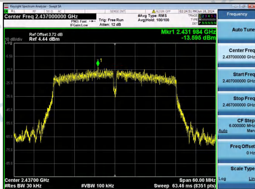
Power_Spectral_Density_NVNT_ANT1_802_11n(HT40)_2437
