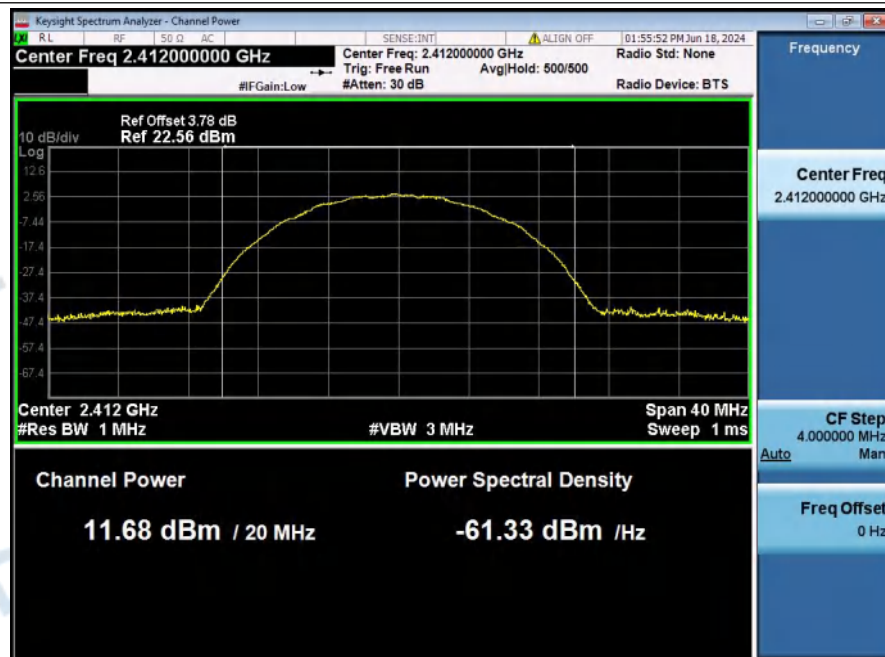
MAX_Output_Power_NVNT_ANT1_802_11b_2412
