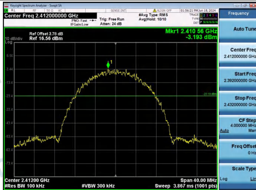
2_Spurious_Emission_NVNT_ANT1_802_11b_2412
