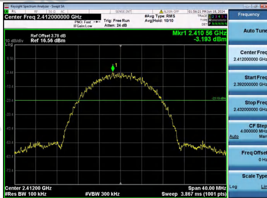
2_Bandedge_NVNT_ANT1_802_11b_2412
