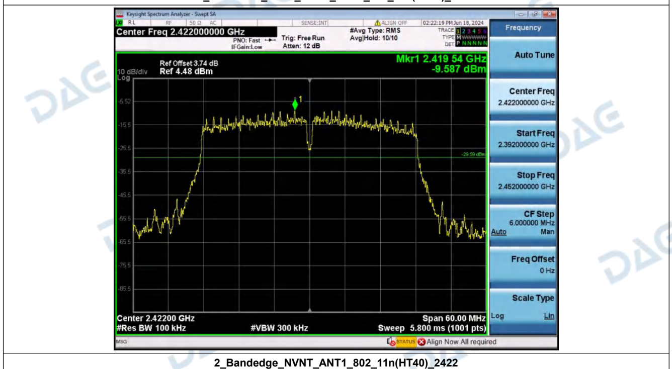
1_Reference_Level_NVNT_ANT1_802_11n(HT40)_2422
