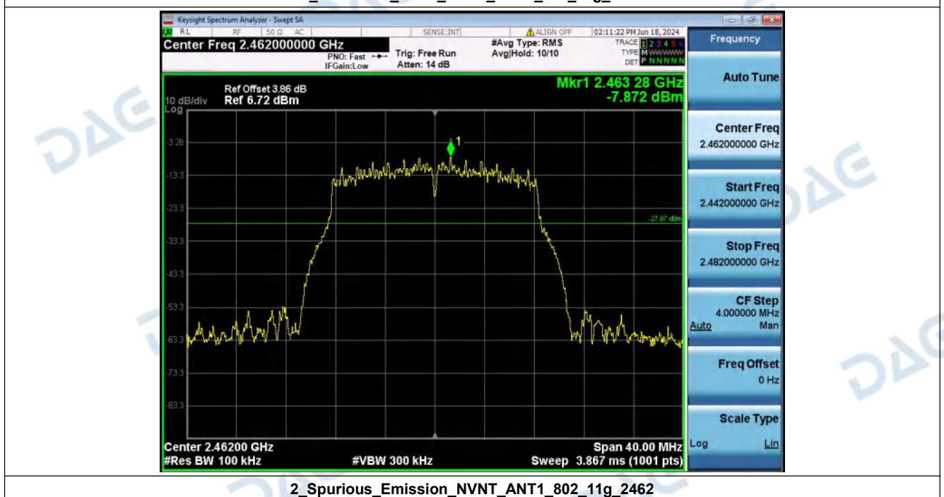
1_Reference_Level_NVNT_ANT1_802_11g_2462
