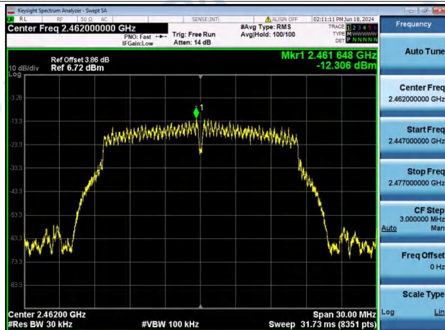
Power_Spectral_Density_NVNT_ANT1_802_11g_2462
