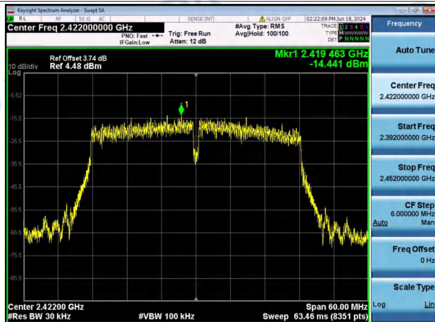
Power_Spectral_Density_NVNT_ANT1_802_11n(HT40)_2422
