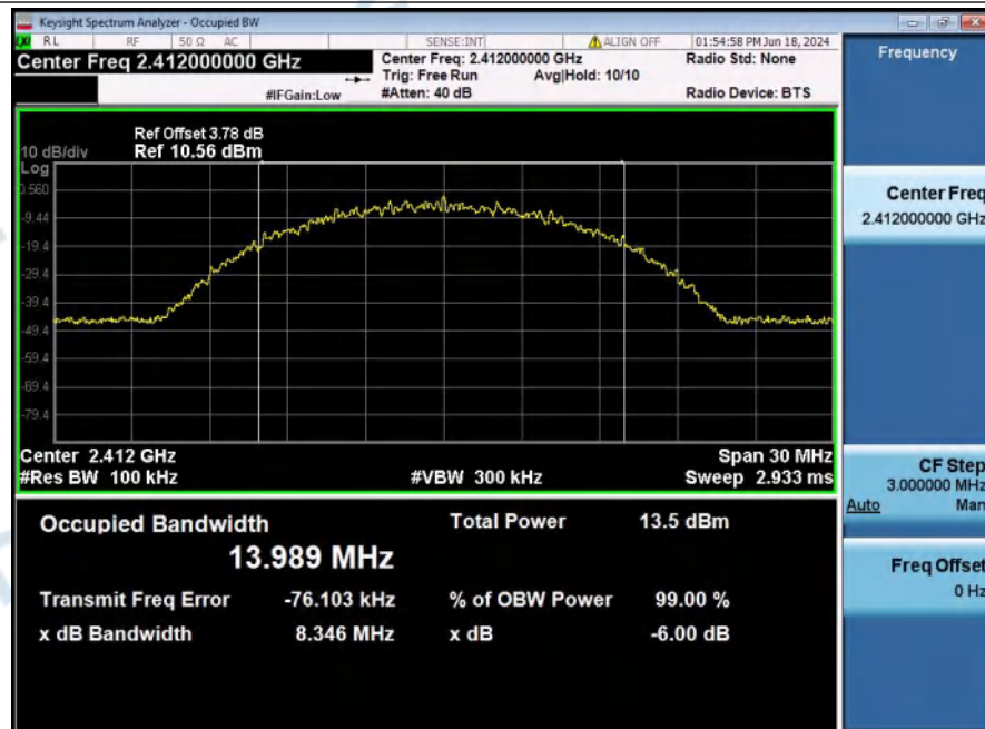
-6dB_Bandwidth_NVNT_ANT1_802_11b_2412
