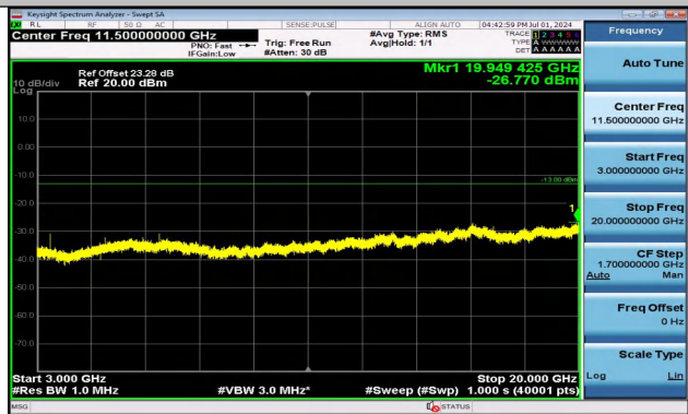
Band4_15MHz_QPSK_20025_1RB#0_3000~20000_3000~20000
