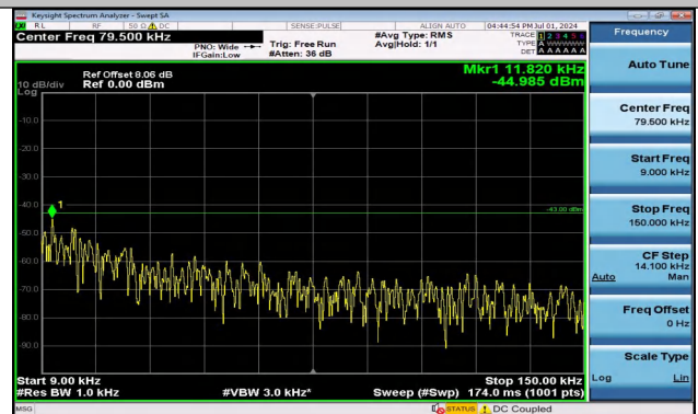
Band4_15MHz_16QAM_20175_1RB#0_0.009~0.15_0.009 ~0.15
