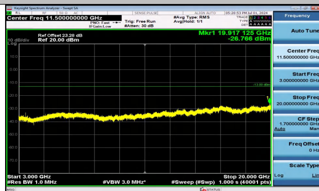
Band4_20MHz_QPSK_20175_1RB#0_3000~20000_3000 ~20000
