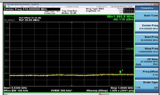
Band4_15MHz_16QAM_20175_1RB#0_30~1000_30~100
