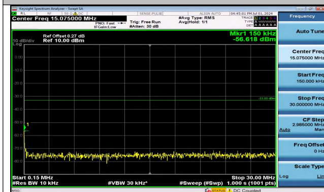
Band4_15MHz_16QAM_20175_1RB#0_0.15~30_0.15~3
