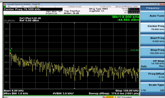
Band4_20MHz_16QAM_20175_1RB#0_0.009~0.15_0.009 ~0.15
