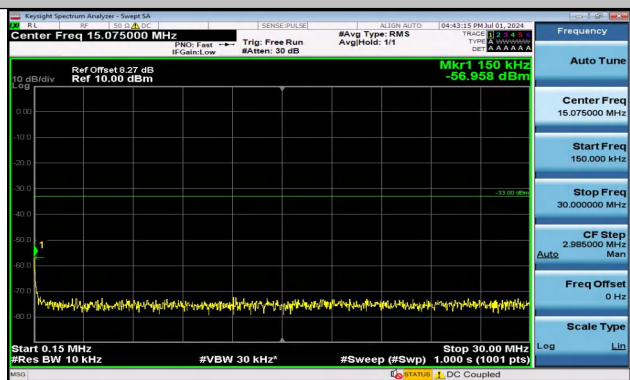
Band4_15MHz_16QAM_20025_1RB#0_0.15~30_0.15~30
