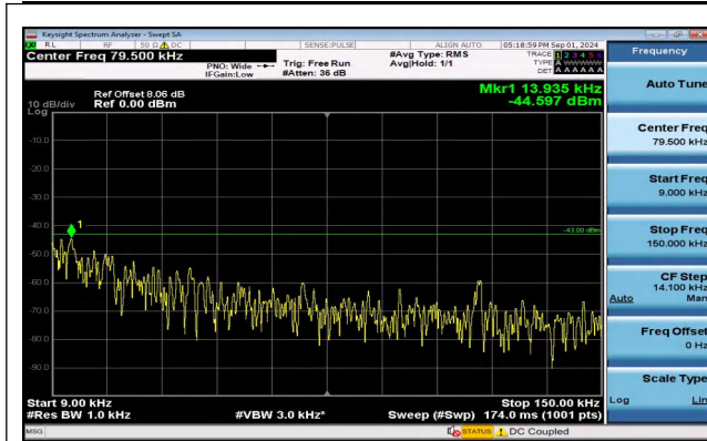
Band4_15MHz_QPSK_20175_1RB#0_0.009~0.15_0.009 ~0.15
