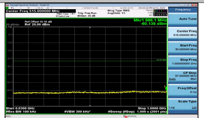
Band4_15MHz_16QAM_20025_1RB#0_30~1000_30~1000
