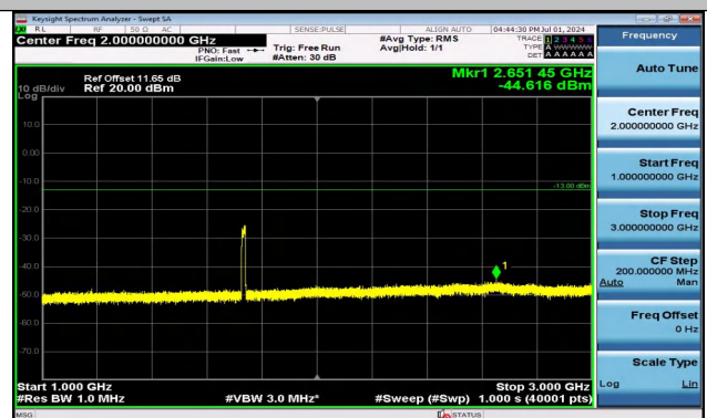
Band4_15MHz_QPSK_20175_1RB#0_1000~3000_1000~3000
