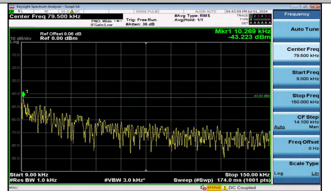
Band4_15MHz_16QAM_20025_1RB#0_0.009~0.15_0.009~0.15
