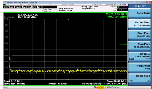
Band4_15MHz_QPSK_20175_1RB#0_0.15~30_0.15~30
