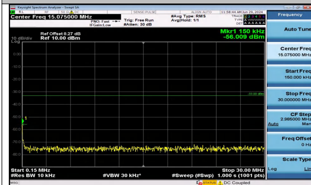
Band2_5MHz_16QAM_19175_1RB#0_0.15~30_0.15~30
