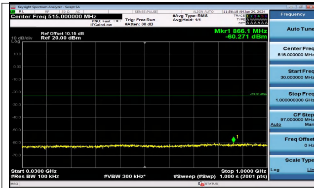
Band2_5MHz_QPSK_18900_1RB#0_30~1000_30~1000
