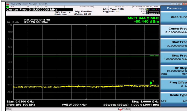
Band2_5MHz_QPSK_19175_1RB#0_30~1000_30~1000
