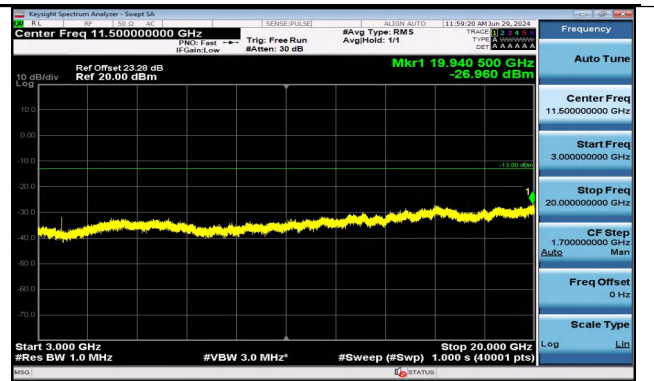
Band2_5MHz_16QAM_19175_1RB#0_3000~20000_3000 ~20000
