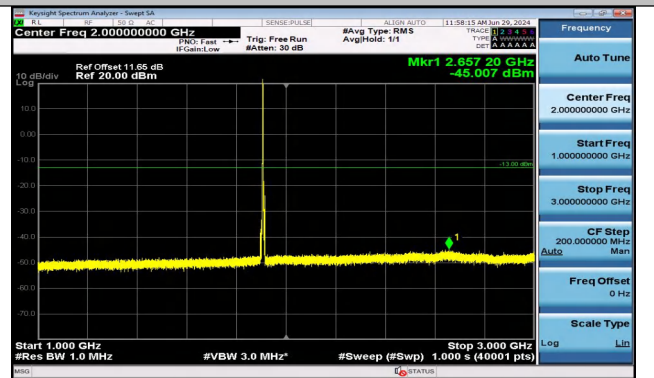
Band2_5MHz_QPSK_19175_1RB#0_1000~3000_1000~3000
