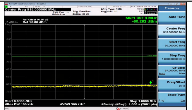
Band2_5MHz_16QAM_18900_1RB#0_30~1000_30~1000
