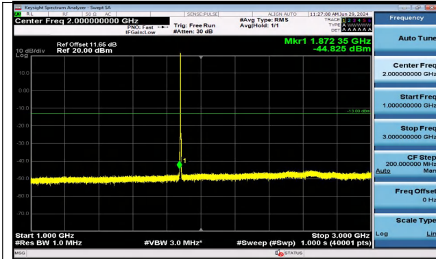
Band2_3MHz_16QAM_18900_1RB#0_1000~3000_1000 ~3000
