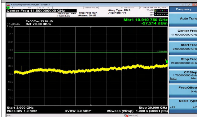
Band2_5MHz_QPSK_19175_1RB#0_3000~20000_3000~20000
