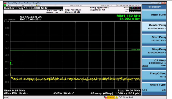
Band2_10MHz_QPSK_18650_1RB#0_0.15~30_0.15~30
