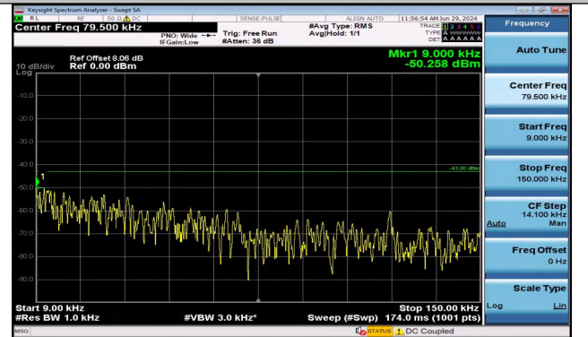
Band2_5MHz_16QAM_18900_1RB#0_0.009~0.15_0.009~0.15
