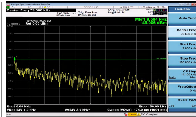
Band2_5MHz_QPSK_19175_1RB#0_0.009~0.15_0.009~0.15
