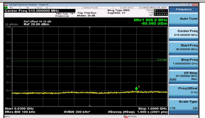
Band2_5MHz_16QAM_19175_1RB#0_30~1000_30~1000
