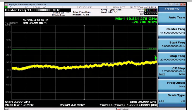
Band2_5MHz_16QAM_18900_1RB#0_3000~20000_3000~20000
