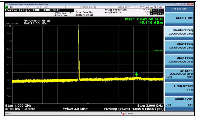
Band2_5MHz_QPSK_18900_1RB#0_1000~3000_1000~3000
