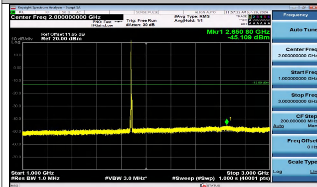
Band2_5MHz_16QAM_18900_1RB#0_1000~3000_1000~3000
