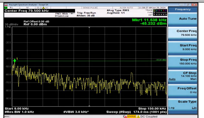
Band2_5MHz_16QAM_19175_1RB#0_0.009~0.15_0.009~0.15
