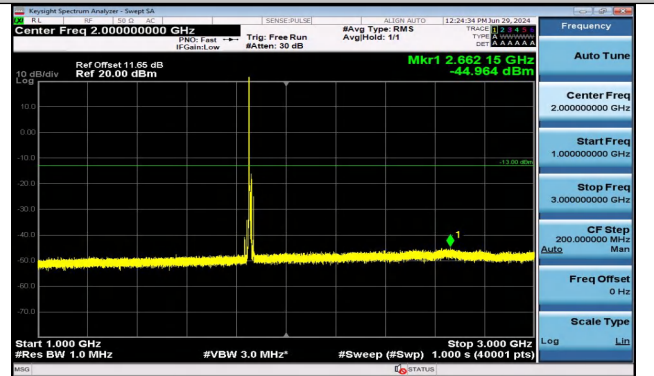
Band2_10MHz_QPSK_18650_1RB#0_1000~3000_1000~3000 000
