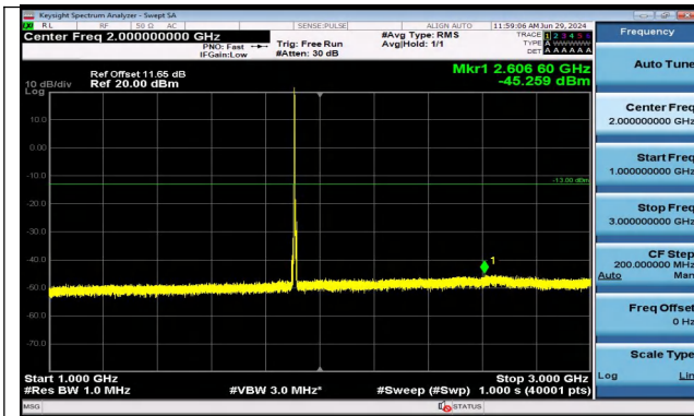
Band2_5MHz_16QAM_19175_1RB#0_1000~3000_1000 ~3000
