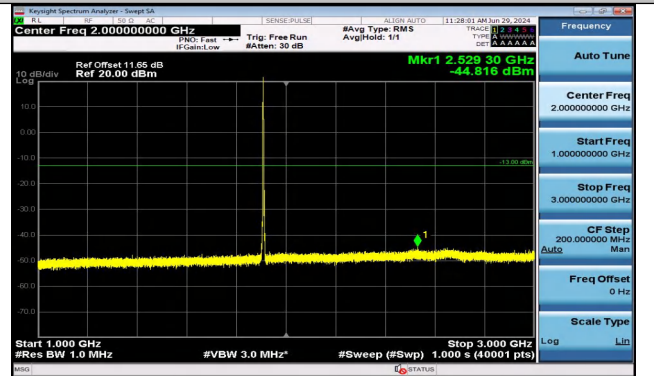
Band2_3MHz_QPSK_19185_1RB#0_1000~3000_1000~3000 00
