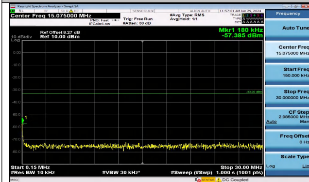
Band2_5MHz_16QAM_18900_1RB#0_0.15~30_0.15~30
