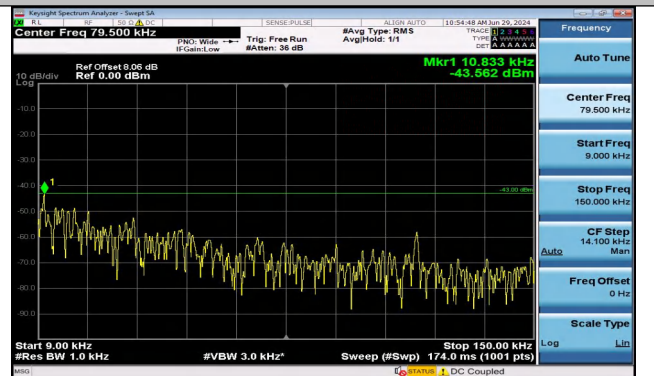
Band2_1.4MHz_16QAM_18900_1RB#0_0.009~0.15_0.009 ~0.15
