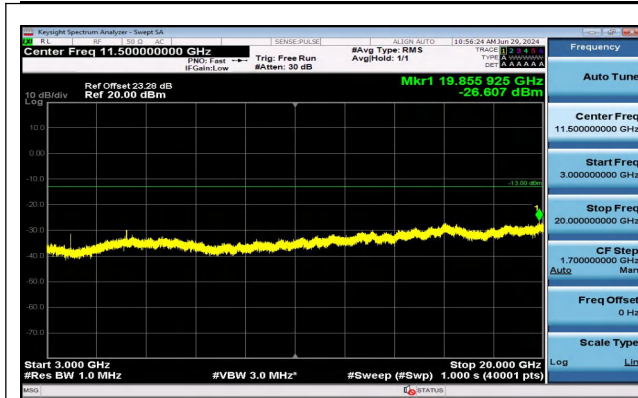
Band2_1.4MHz_QPSK_19193_1RB#0_3000~20000_300 0~20000
