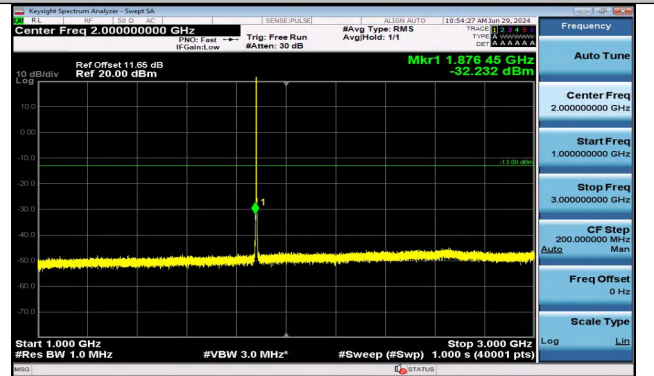
Band2_1.4MHz_QPSK_18900_1RB#0_1000~3000_1000~3000
