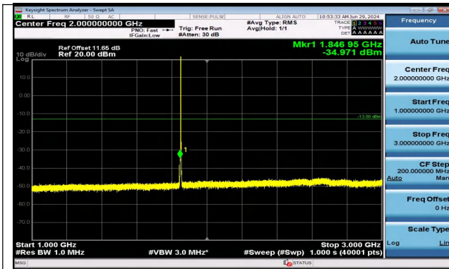
Band2_1.4MHz_16QAM_18607_1RB#0_1000~3000_100 0~3000
