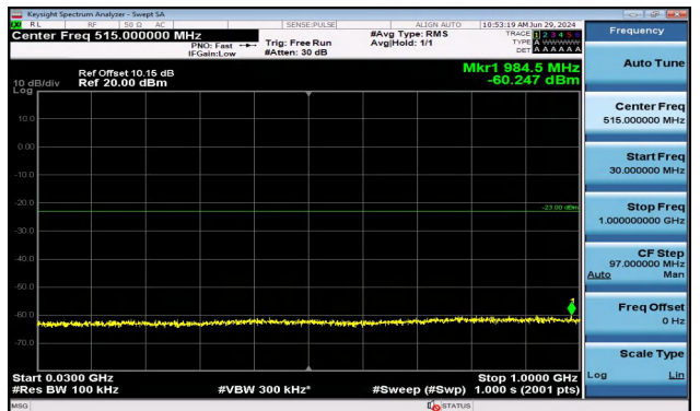
Band2_1.4MHz_16QAM_18607_1RB#0_30~1000_30~1000
