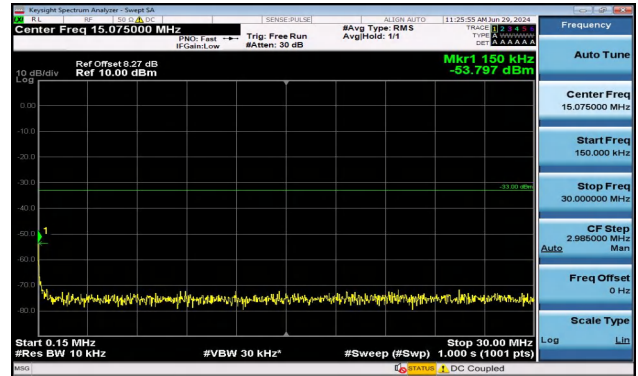
Band2_3MHz_QPSK_18900_1RB#0_0.15~30_0.15~30
