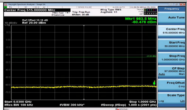
Band2_3MHz_16QAM_18900_1RB#0_30~1000_30~1000
