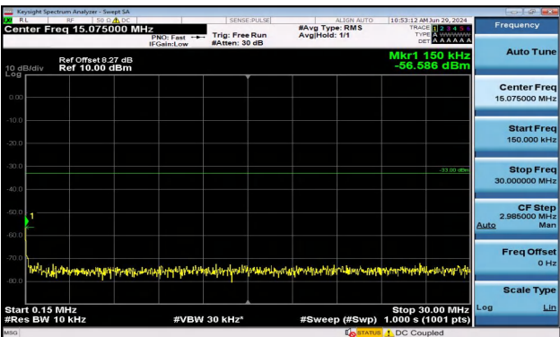
Band2_1.4MHz_16QAM_18607_1RB#0_0.15~30_0.15~30
