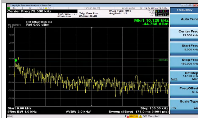
Band2_3MHz_QPSK_18615_1RB#0_0.009~0.15_0.009~
