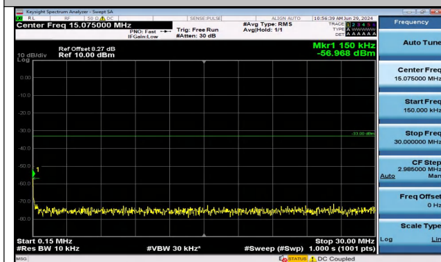
Band2_1.4MHz_16QAM_19193_1RB#0_0.15~30_0.15~3 0
