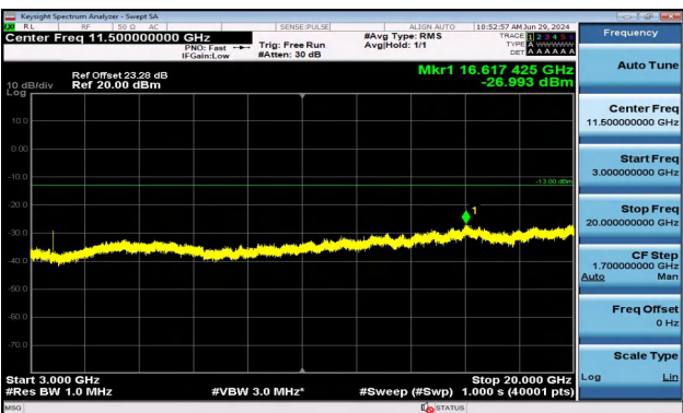
Band2_1.4MHz_QPSK_18607_1RB#0_3000~20000_3000~20000
