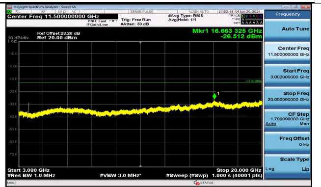
Band2_1.4MHz_16QAM_18607_1RB#0_3000~20000_300 0~20000
