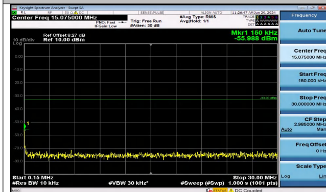
Band2_3MHz_16QAM_18900_1RB#0_0.15~30_0.15~30
