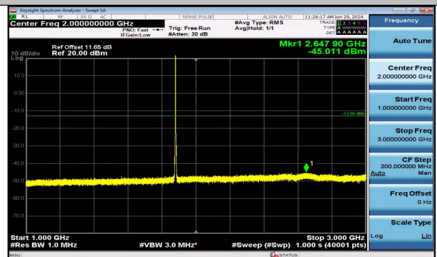
Band2_3MHz_QPSK_18900_1RB#0_1000~3000_1000~3000
