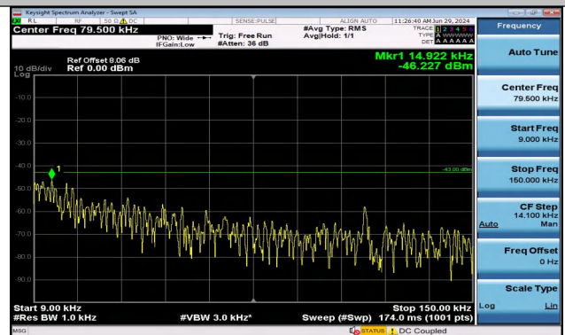
Band2_3MHz_16QAM_18900_1RB#0_0.009~0.15_0.009~0.15
