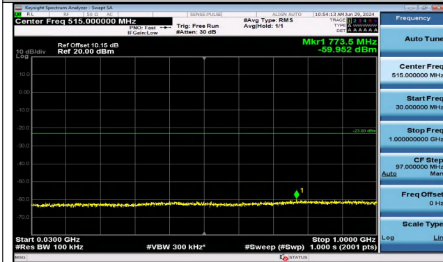
Band2_1.4MHz_QPSK_18900_1RB#0_30~1000_30~100 0
