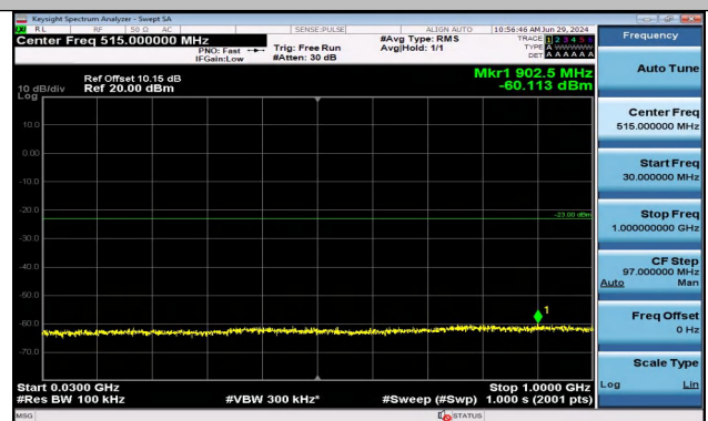
Band2_1.4MHz_16QAM_19193_1RB#0_30~1000_30~100 0
