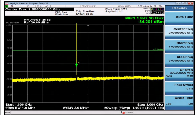
Band2_1.4MHz_QPSK_18607_1RB#0_1000~3000_1000~3000
