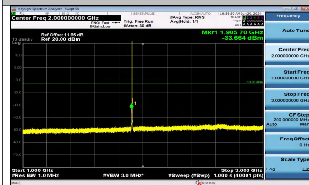
Band2_1.4MHz_16QAM_19193_1RB#0_1000~3000_100 0~3000
