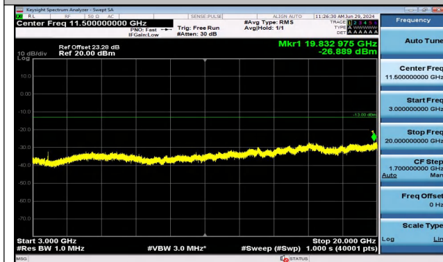
Band2_3MHz_QPSK_18900_1RB#0_3000~20000_3000~20000
