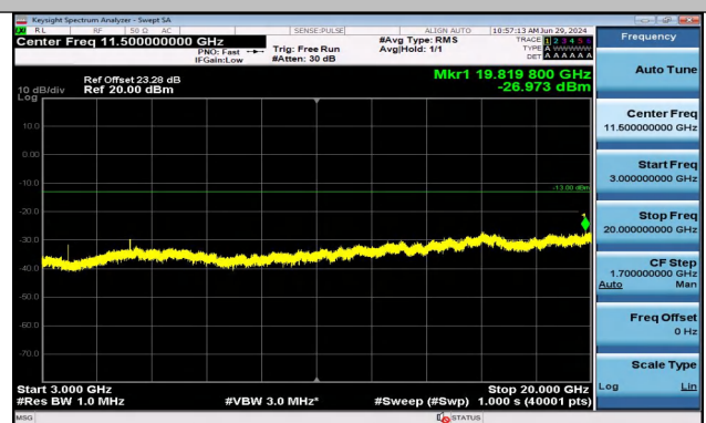
Band2_1.4MHz_16QAM_19193_1RB#0_3000~20000_300 0~20000
