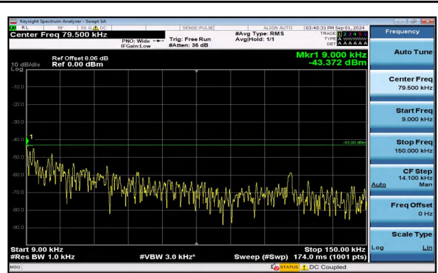
Band2_1.4MHz_16QAM_19193_1RB#0_0.009~0.15_0.009 ~0.15
