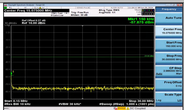
Band2_3MHz_QPSK_18615_1RB#0_0.15~30_0.15~30
