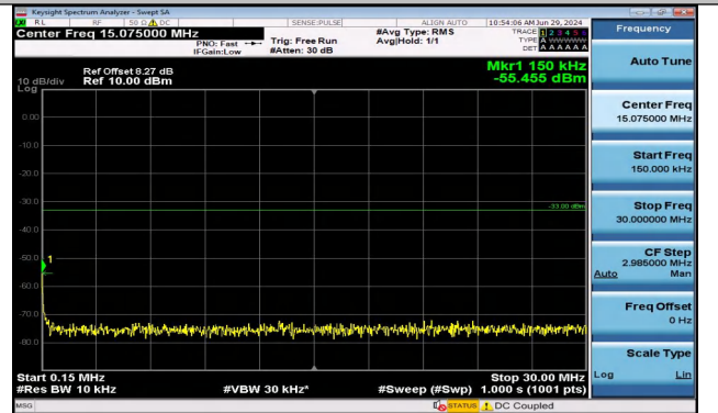
Band2_1.4MHz_QPSK_18900_1RB#0_0.15~30_0.15~30
