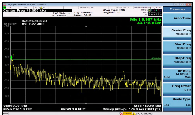
Band2_1.4MHz_16QAM_18607_1RB#0_0.009~0.15_0.009~0.15
