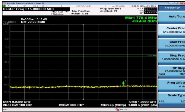
Band2_1.4MHz_QPSK_18607_1RB#0_30~1000_30~1000
