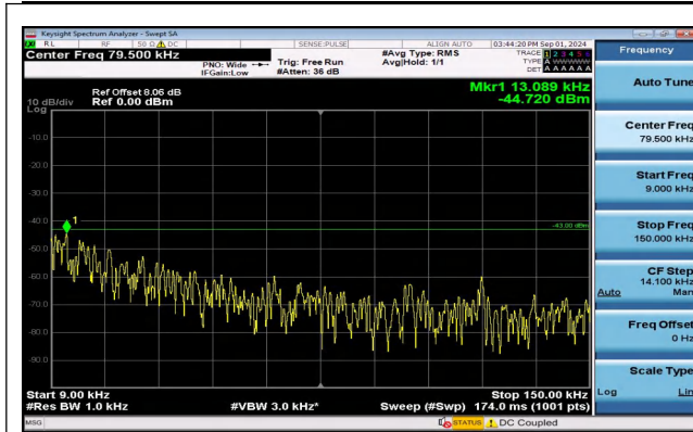
Band2_3MHz_QPSK_18900_1RB#0_0.009~0.15_0.009~0.15
