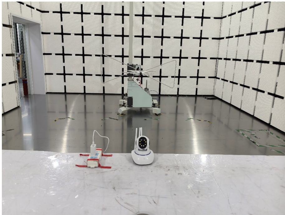
Radiated Emission
