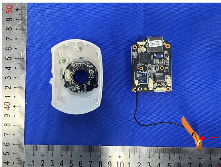
WIFI Antenna
