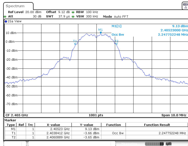
Thread_Ant1_2405
