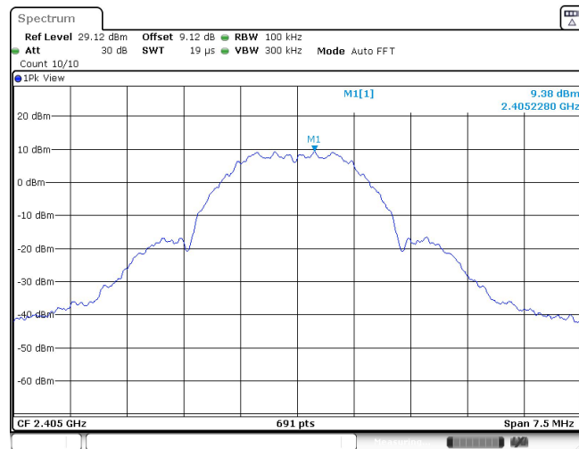
Thread_Ant1_2405_0~Reference
