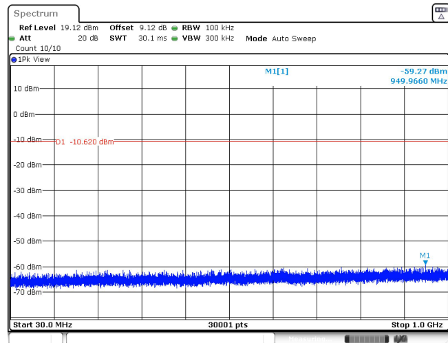
Thread_Ant1_2405_30~1000
