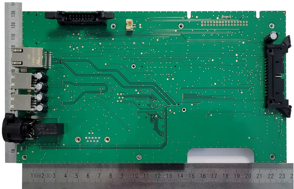
Figure 4: HighLevel PCB, bottom view
