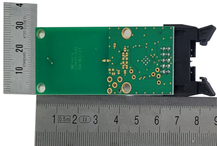
Figure 8: RFID Read-Writer PCB, bottom view
