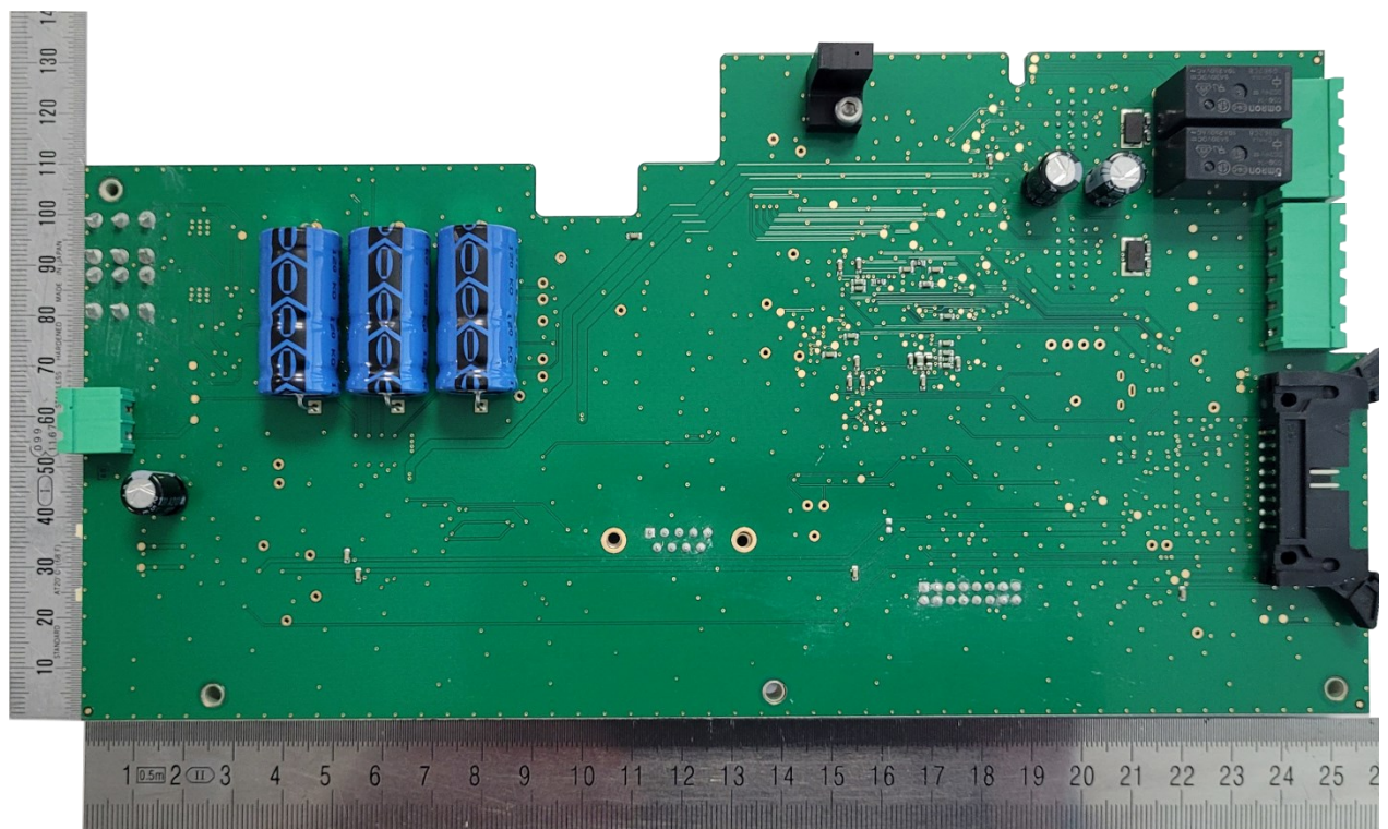
Figure 6: LowLevel PCB, bottom view
