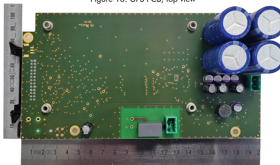
Figure 14: UPS PCB, bottom view
