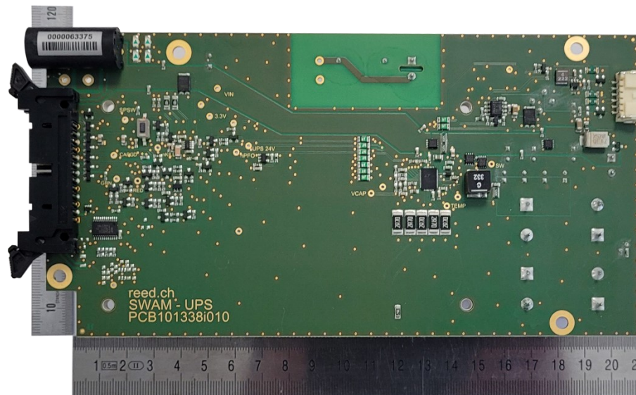
Figure 13: UPS PCB, top view
