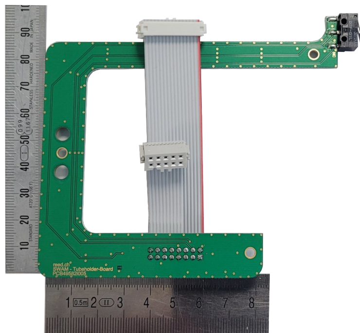
Figure 12: Tubeholder PCB, bottom view
