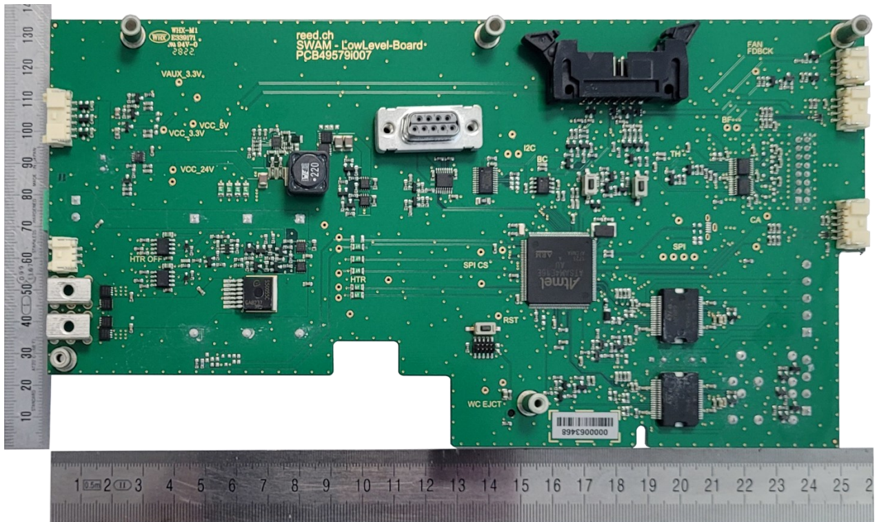
Figure 5: LowLevel PCB, top view
