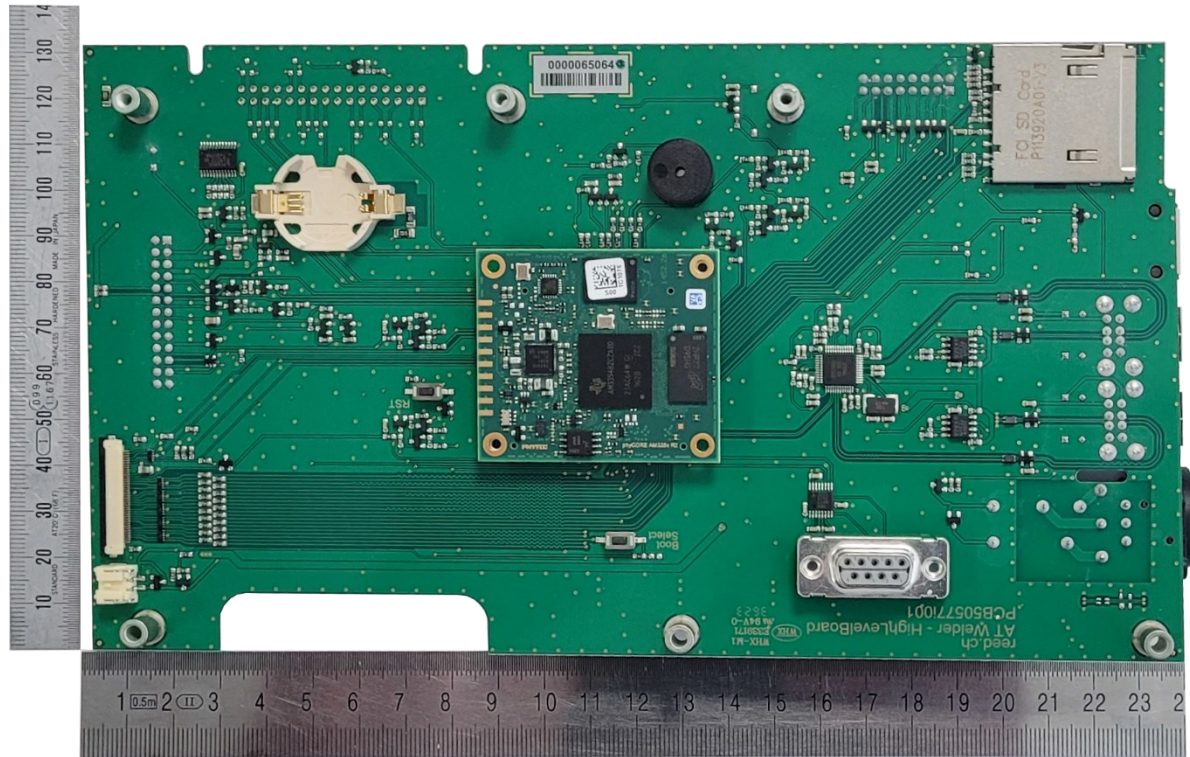
Figure 3: HighLevel PCB, top view
