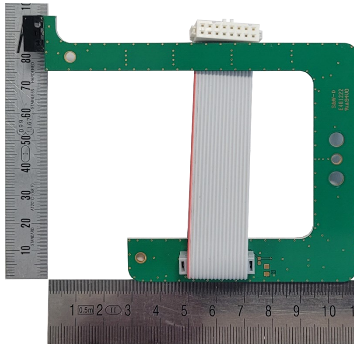
Figure 11: Tubeholder PCB, top view
