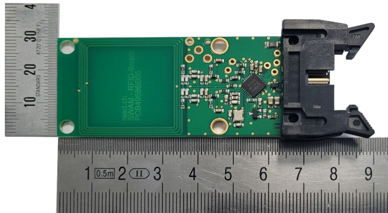
Figure 7: RFID Read-Writer PCB, top view
