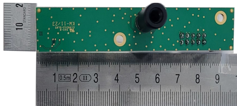
Figure 10: Thermopile PCB, bottom view
