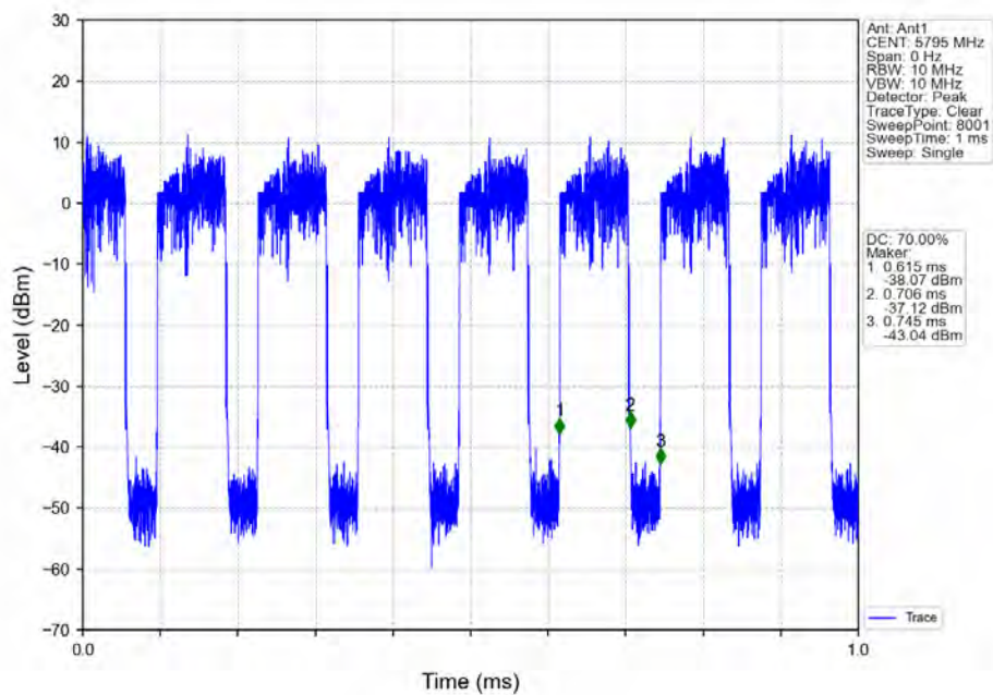
802.11ac(VHT40)_HCH_5795MHz_Ant1_NTNV
