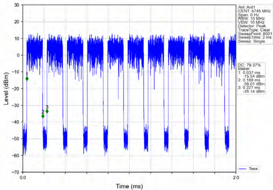
802.11ac(VHT20)_LCH_5745MHz_Ant1_NTNV
