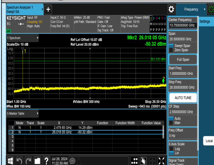
BLE_1M-Ant1-2480-1000~26500-PASS
