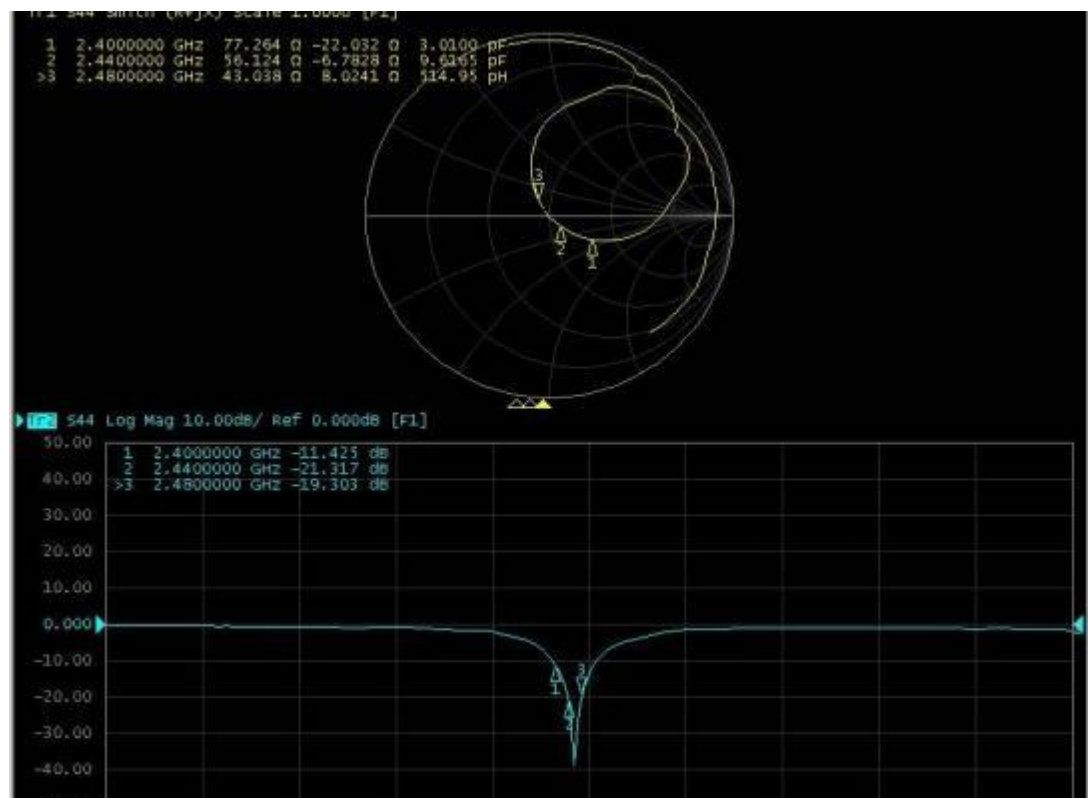
Return Loss
