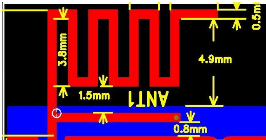
3-1NormalModuleWiggleAntenna
