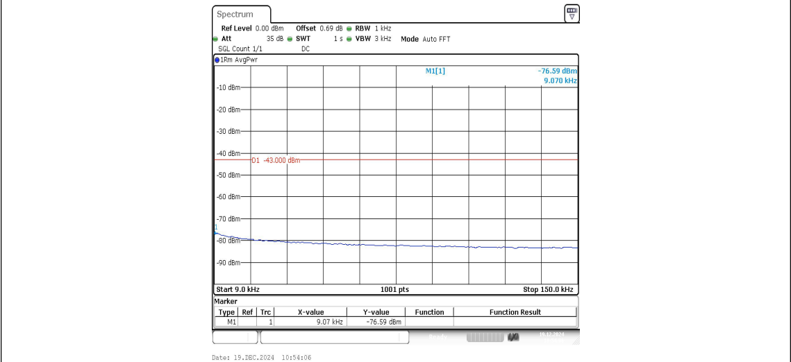
Band2-9538-0.009~0.15MHz-PASS
