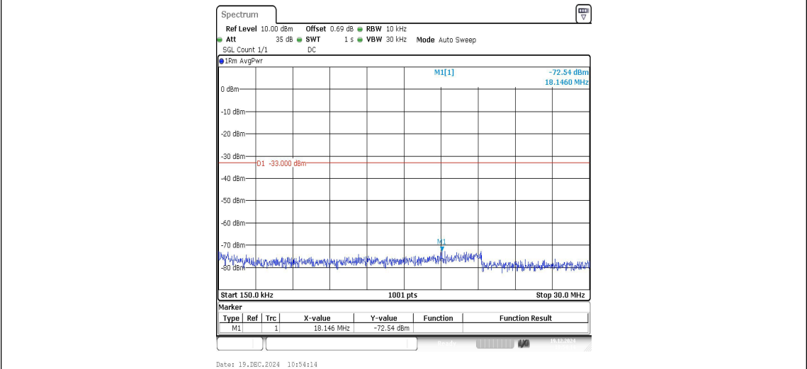
Band2-9538-0.15~30MHz-PASS
